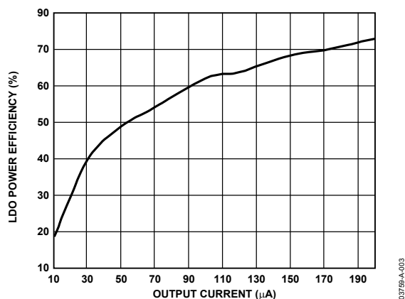
Figure 3. LDO Efficiency in Blanking Mode with V_{CC} = 3\text{ V}
