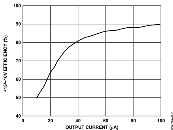
Figure 8. +15 V/-10 V Efficiency vs. Output Current in Scanning Mode, V_{CC} = 3\text{ V}
