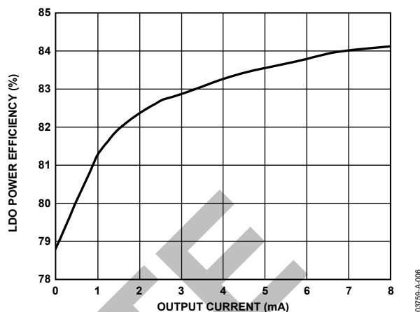
Figure 6. LDO Efficiency in Scanning Mode with V_{CC} = 3\text{ V}
