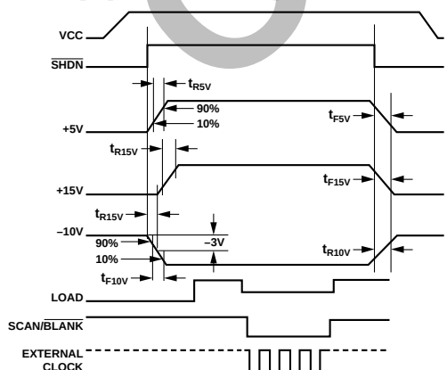
Figure 17. Power Sequence
