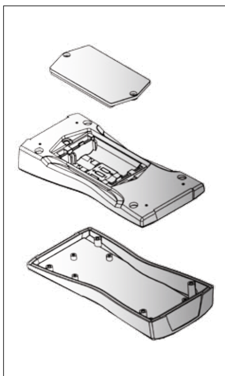
BS .01, with battery compartment, IP 40
