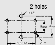
Drill-hole diagram
