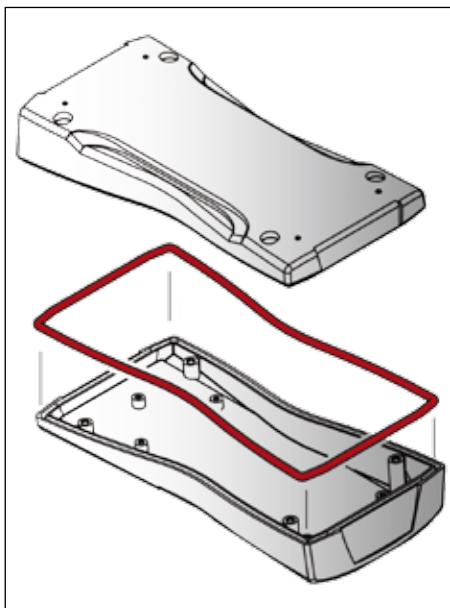
BS .02, without battery compartment, IP 65
