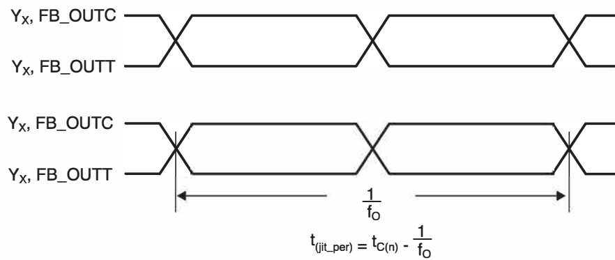
Figure 6. Period Jitter
