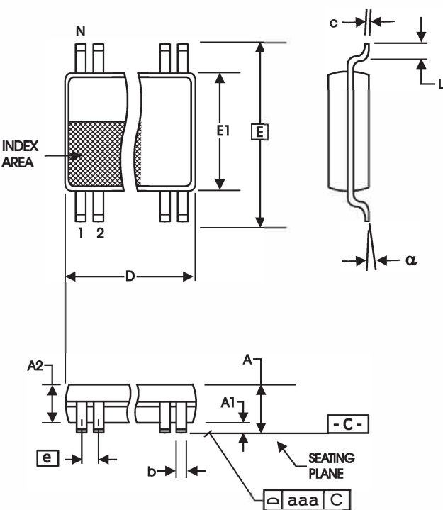
6.10 mm. Body, 0.50 mm. pitch TSSOP (240 mil) (0.020 mil)
