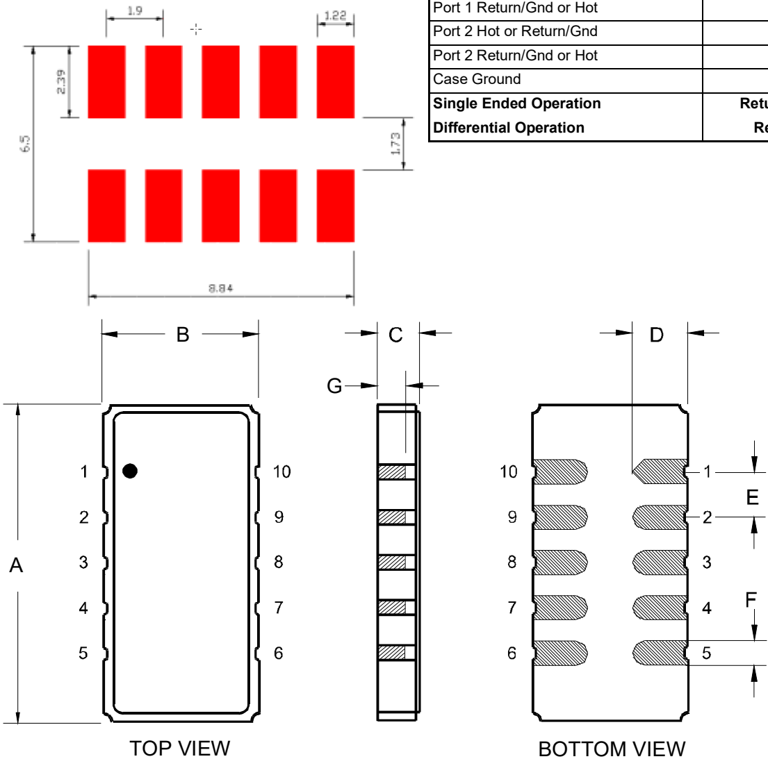
Typical PCB Land Pattern
