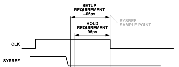
Figure 121. SYSREF High to Low Transition Using Falling Edge Clock Capture (Register 0x0120, Bit 4 = 1'b1, Register 0x0120, Bit 3 = 1'b1)
