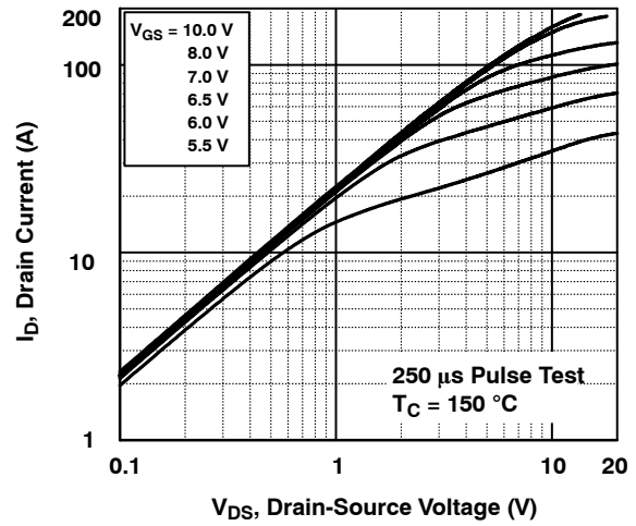
Figure 2. On-Region Characteristics
