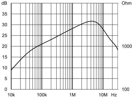
RT8x21-63-4M4
