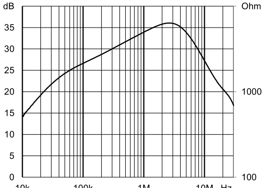
RT8x21-50-8M6
