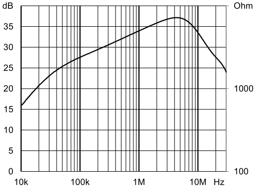
RT8x21-40-10M1
