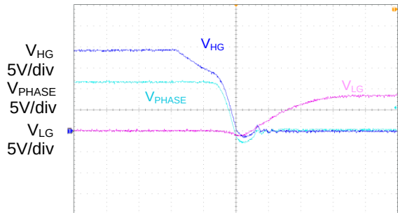
Dead Time 1
