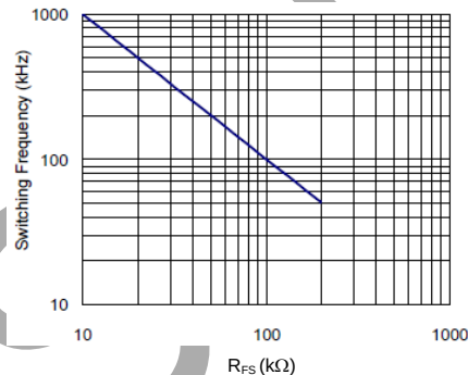
Figure 2. Switching Frequency vs. R_{FS}
