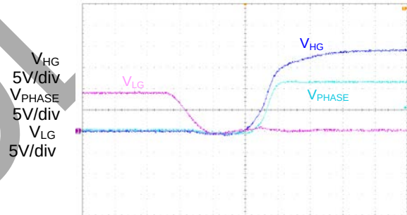
Dead Time 2
