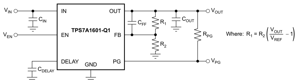
Figure 8-1. TPS7A16-Q1 Circuit as an Adjustable Regulator Schematic
