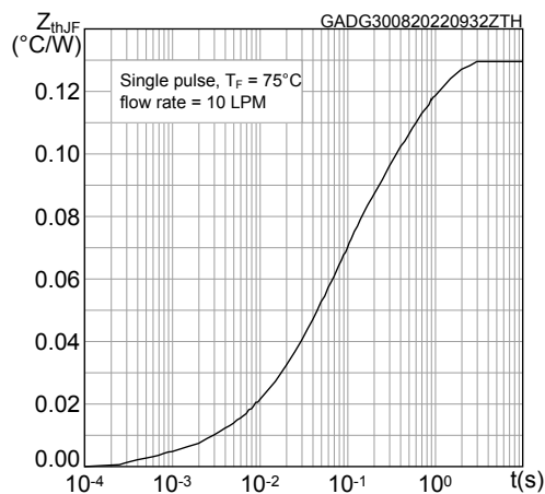
Figure 15. Typical transient thermal impedance
