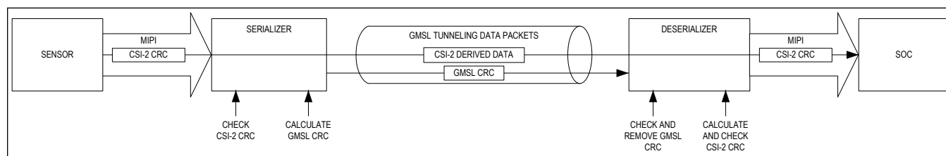
Figure 16. Tunneling Mode
