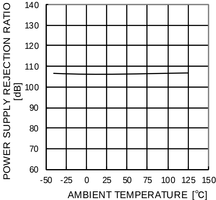
Figure 25. Power Supply Rejection Ratio – Ambient Temperature
