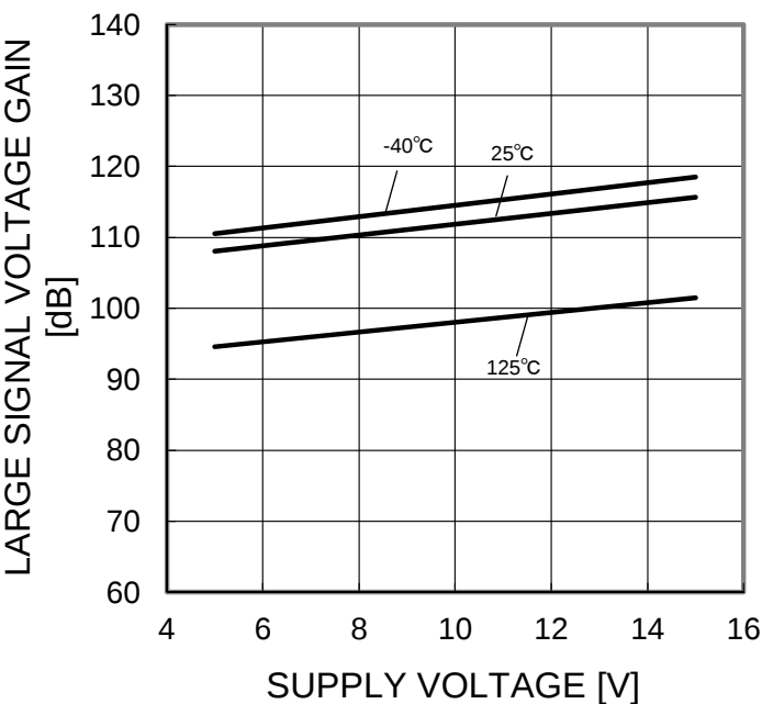
Figure 21. Large Signal Voltage Gain – Supply Voltage (RL=2kΩ)
