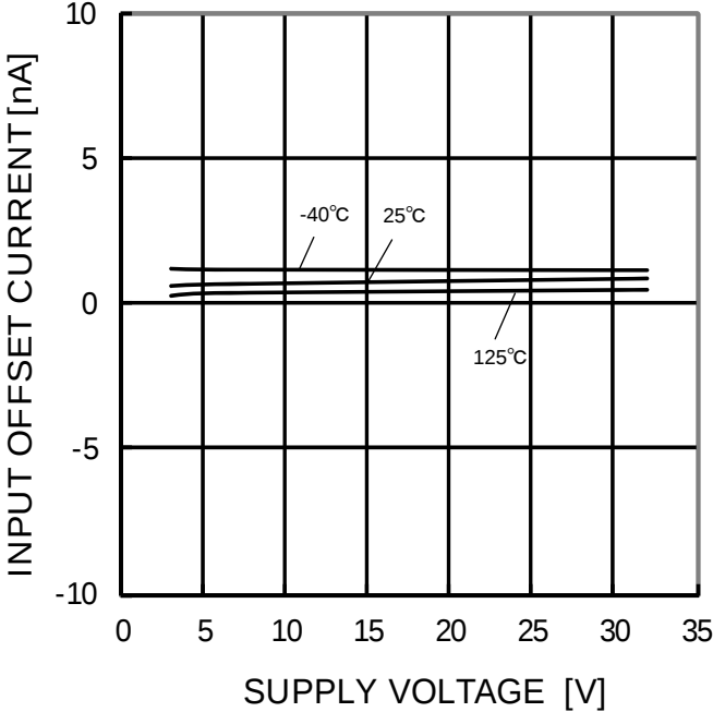
Figure 19. Input Offset Current – Supply Voltage (Vicm=0V, OUT=1.4V)
