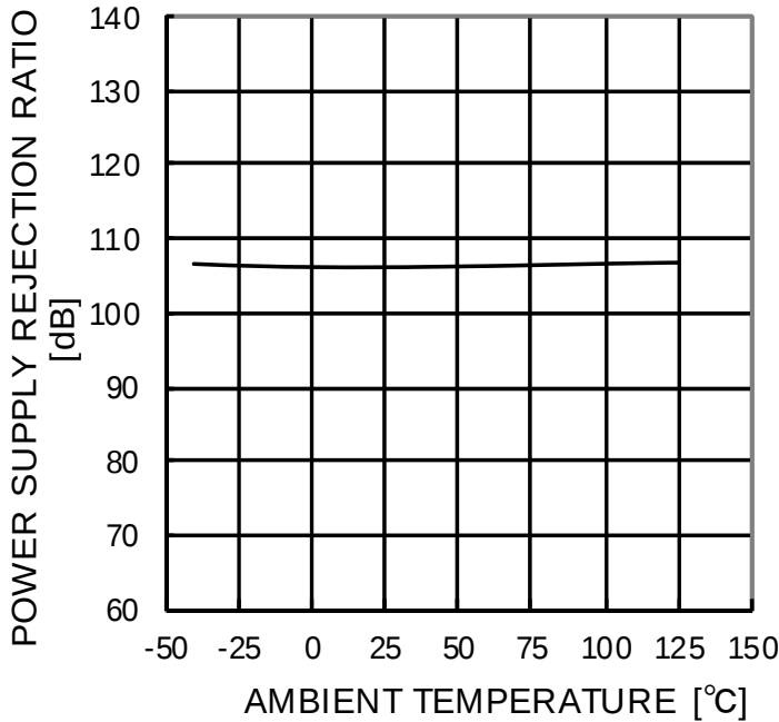
Figure 49. Power Supply Rejection Ratio – Ambient Temperature
