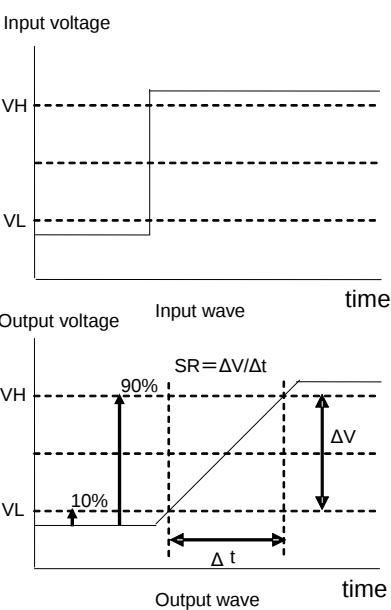
Figure . 54 Slew Rate Input Waveform
