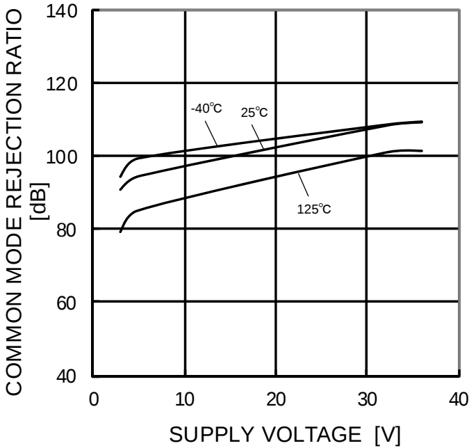
Figure 47. Common Mode Rejection Ratio – Supply Voltage
