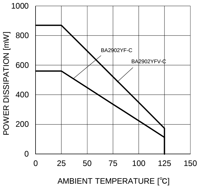
Figure 26. Derating Curve
