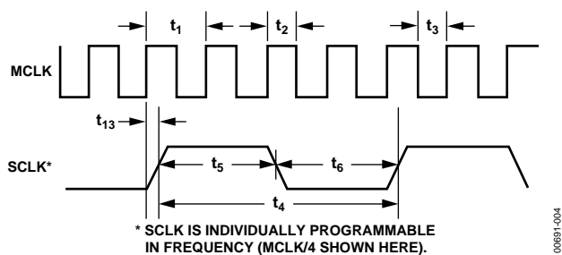
Figure 4. SCLK Timing
