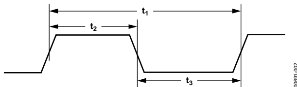
Figure 2. MCLK Timing
