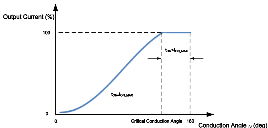
Figure 3. Dimming Curve
