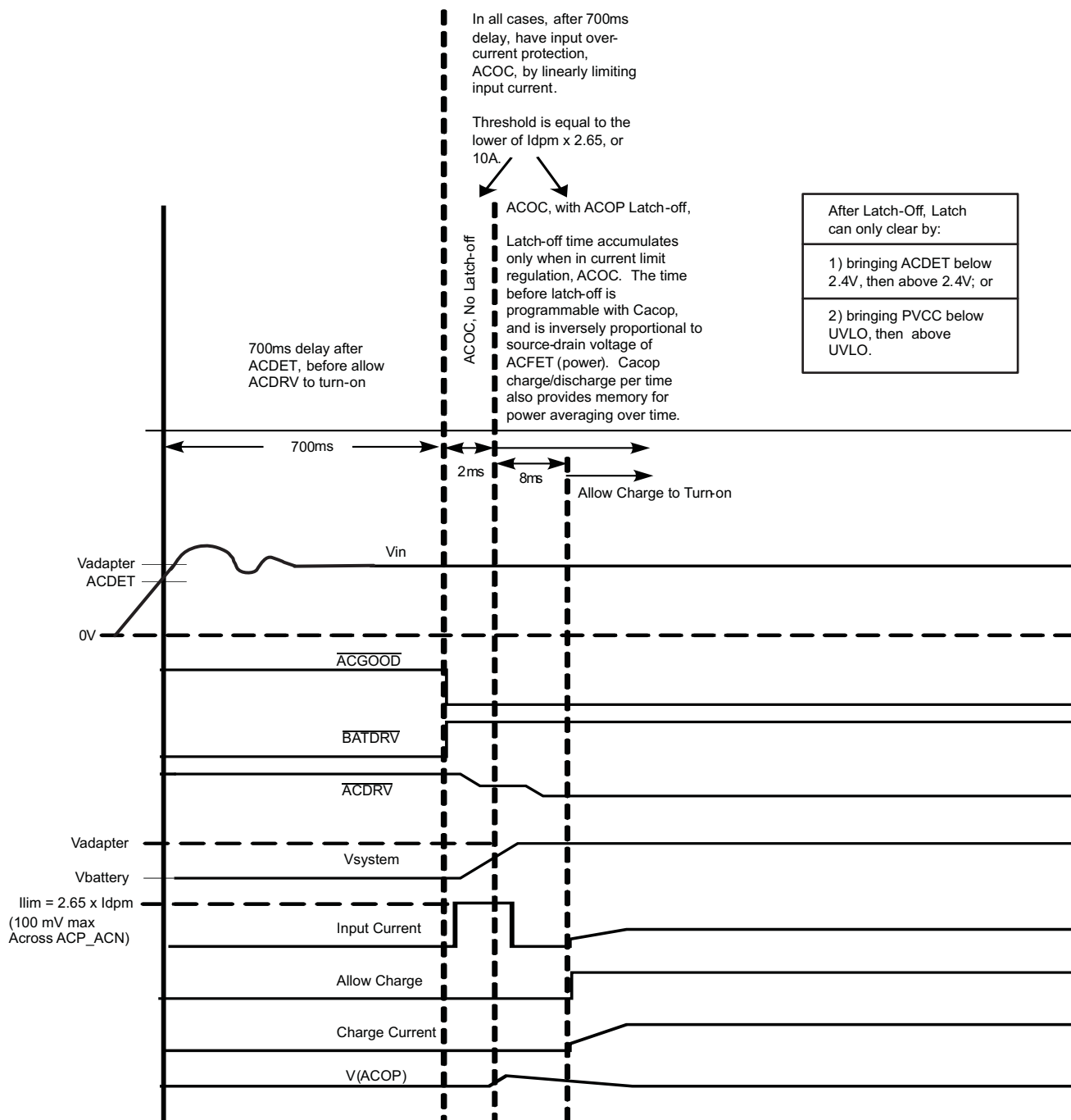
Figure 37. ACOC Protection During Adapter Insertion
