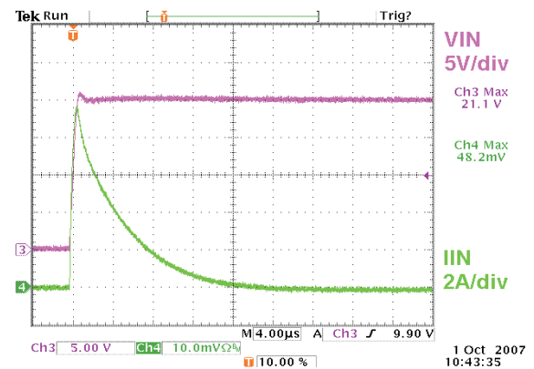
Figure 43. Adapter DC Side Hot Plug-in Test Waveforms
