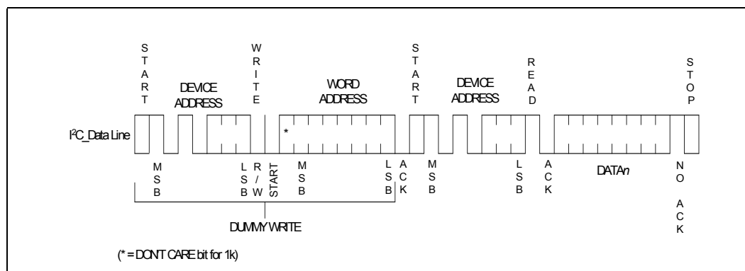
Figure 28 Random Read
