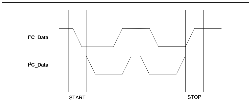
Figure 26 Start and Stop Definition Timing
