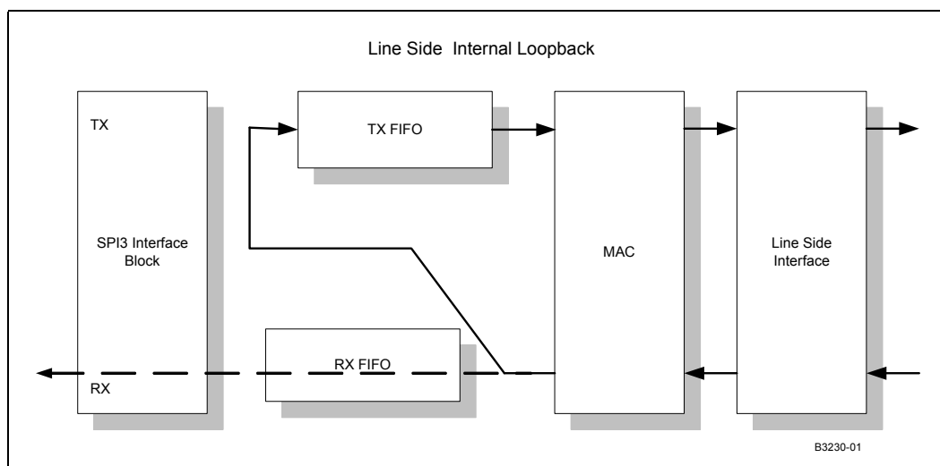
Figure 34 Line Side Interface Loopback Path
