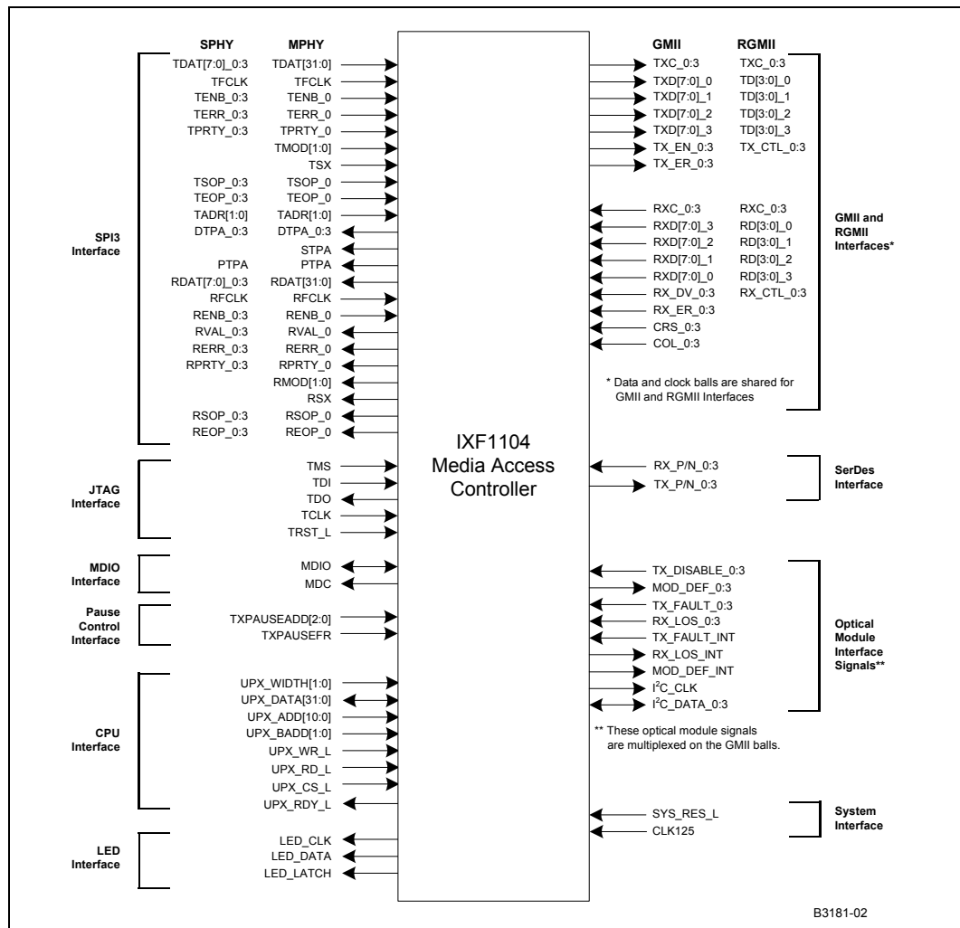
Figure 4 Interface Signals
