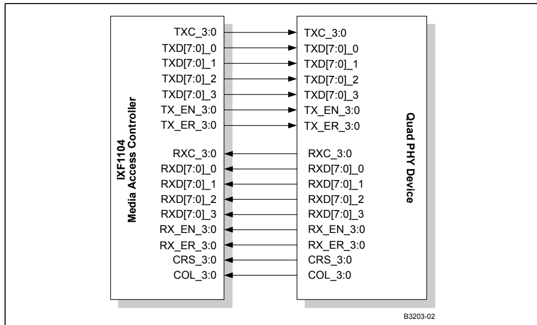
Figure 18 RGMI Interface
