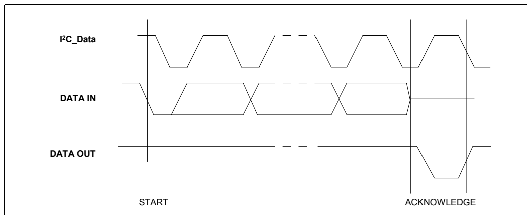
Figure 27 Acknowledge Timing
