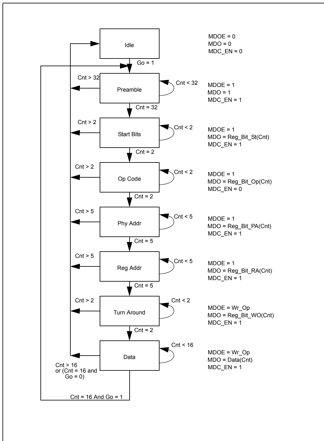
Figure 22 MDI State
