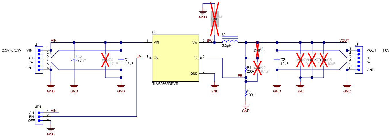
Figure 5. TLV6256xEVM-789 Schematic
