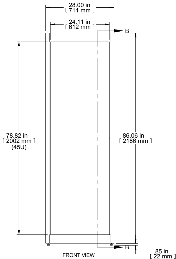
FRONT VIEW
