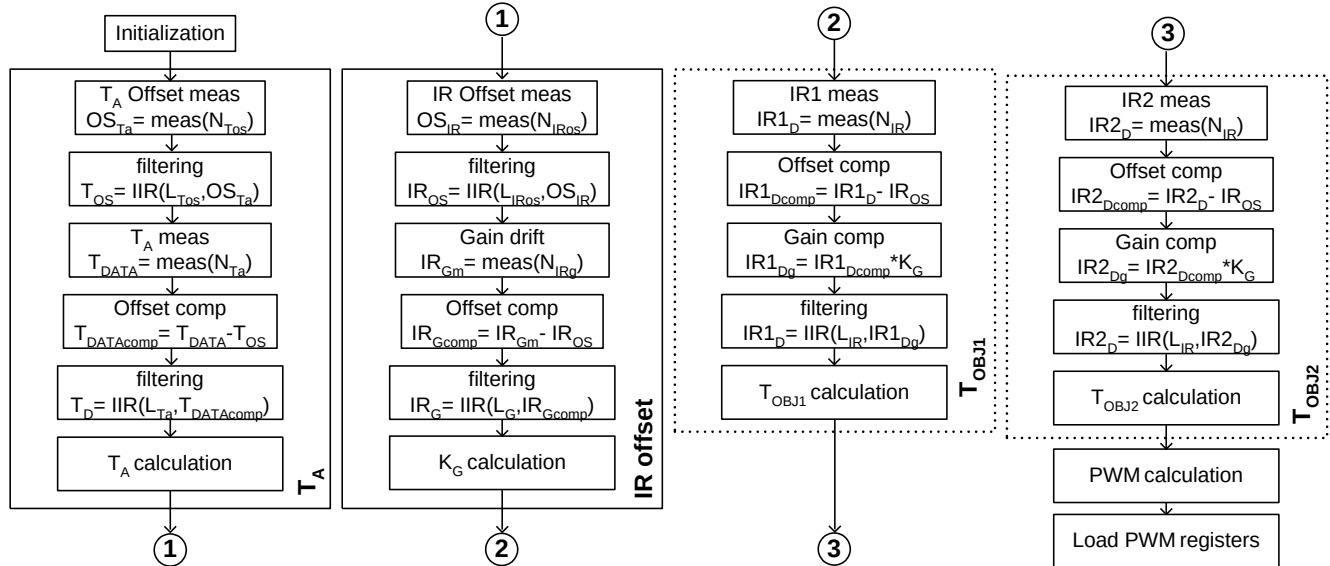
Figure 20 – Software flow
