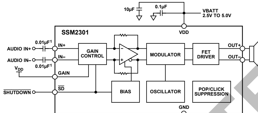
Figure 24. Differential Input Configuration, Gain = 12 dB
