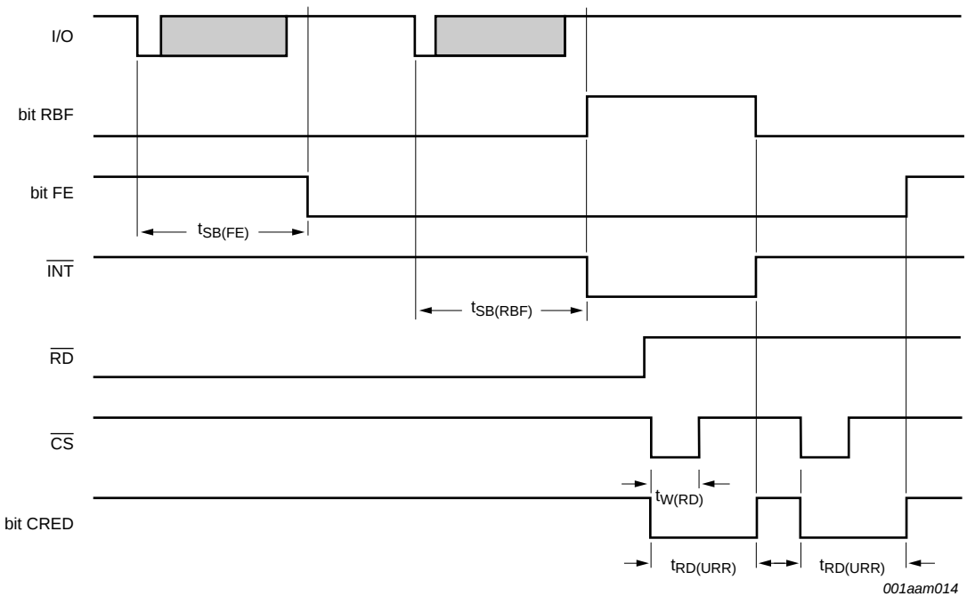
Fig 10. Minimum time between two read operations in register URR - non-multiplexed bus
