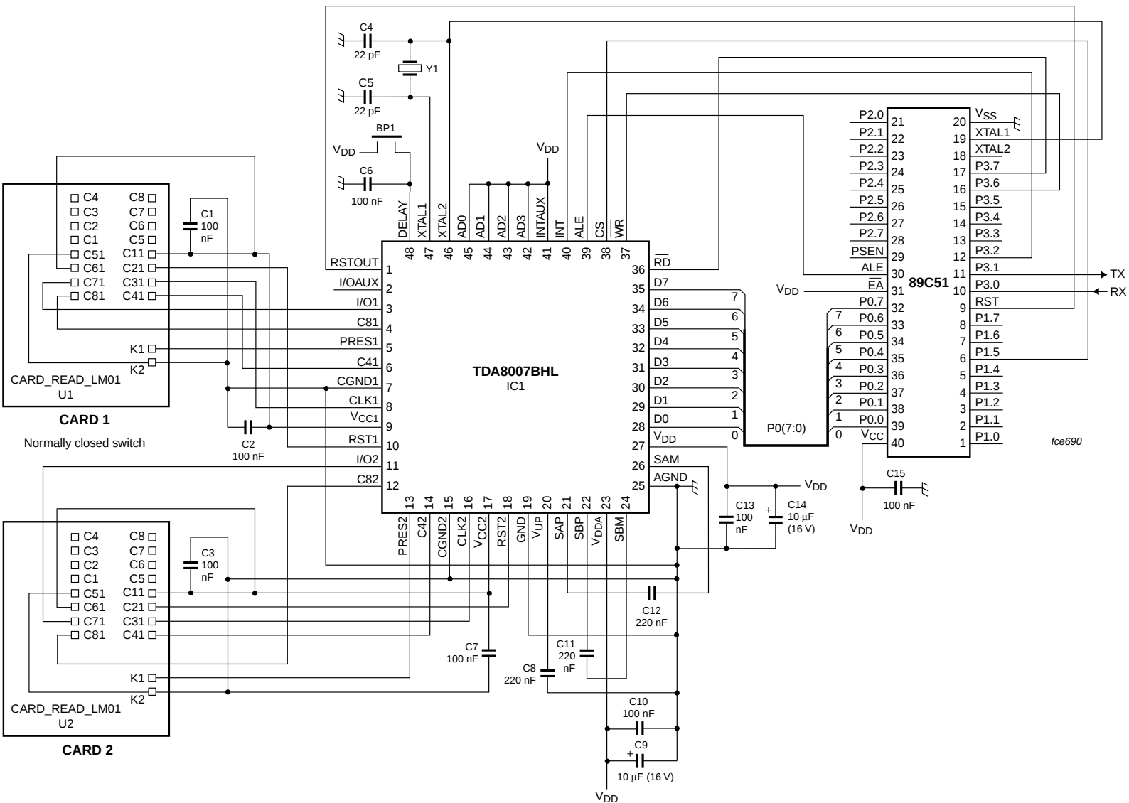
Fig 21. TDA8007BHL/C3 application
