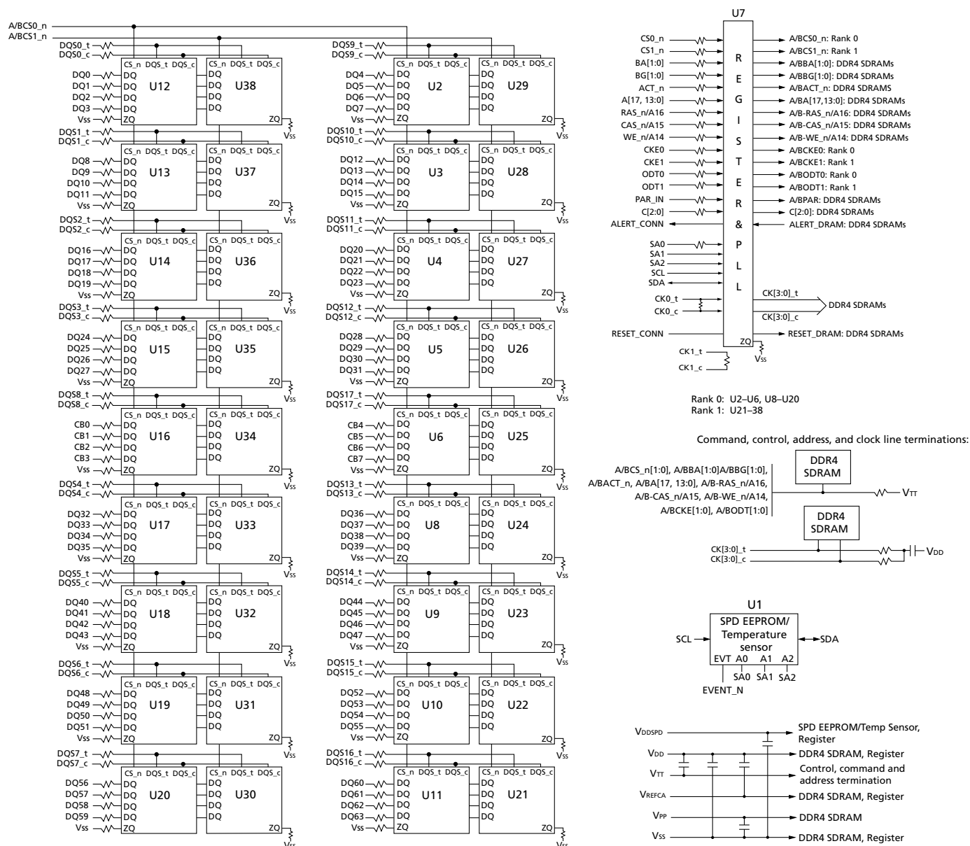
Figure 4: Functional Block Diagram (R/C-B2, PCB 1971, PCB 2364, PCB 2436)
