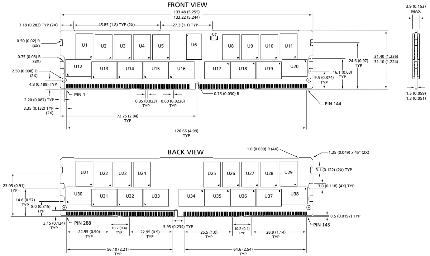
Figure 5: 288-Pin DDR4 RDIMM (R/C-B1, PCB 1798, PCB 1870)
