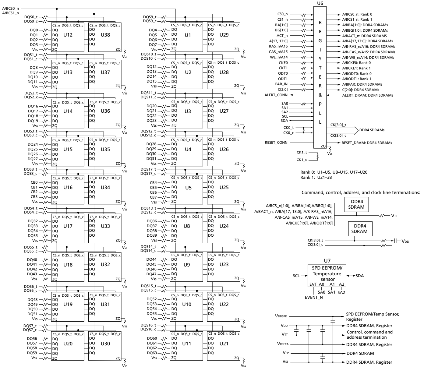
Figure 3: Functional Block Diagram (R/C-B1, PCB 1798, PCB 1870)
