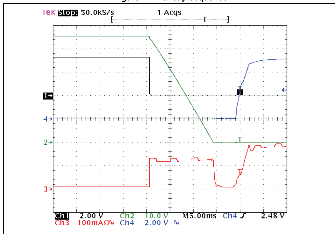
Figure 12. Wakeup sequence
