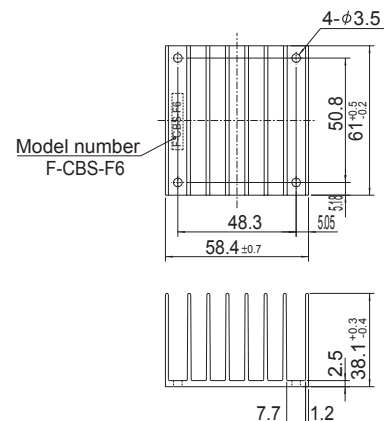
Fig.6 F-CBS-F6 external view
