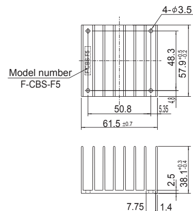
Fig.3 F-CBS-F5 external view
