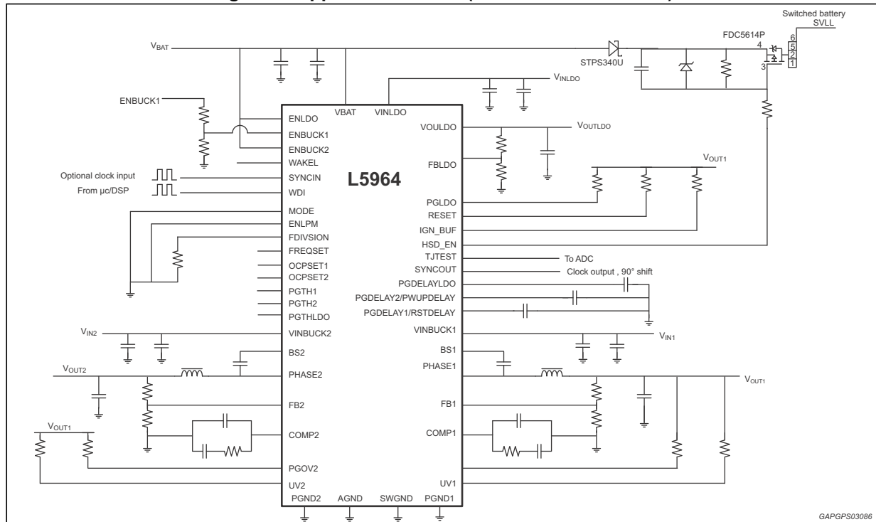
Figure 4. Application circuit (microcontroller mode)
