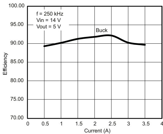
Figure 6. Efficiency at 250 kHz ( V_{in} = 14 \text{ V} , V_{out} = 5 \text{ V} )
