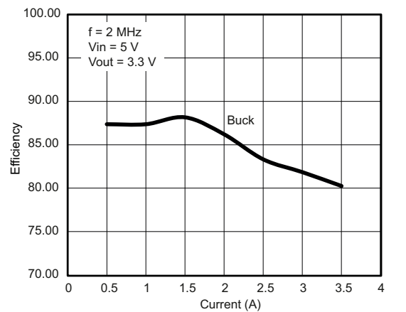
Figure 7. Efficiency at 2 MHz ( V_{in} = 5 \text{ V} , V_{out} = 3.3 \text{ V} )
