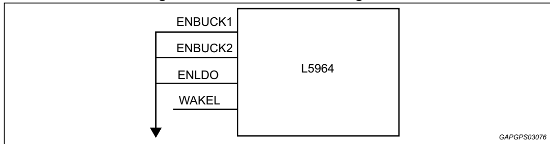
Figure 12. Shutdown Mode configuration
