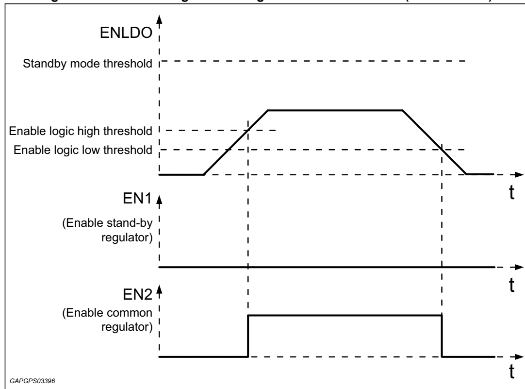
Figure 10. Enable timing for LDO regulator in Normal Mode (ENLDO &lt; 5 V)
