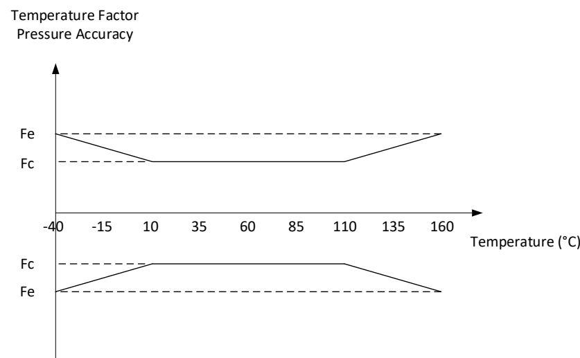
Figure 7: Pressure accuracy temperature factor (G temperature code)
