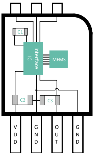
Figure 2: Internal wiring of MLX90823
