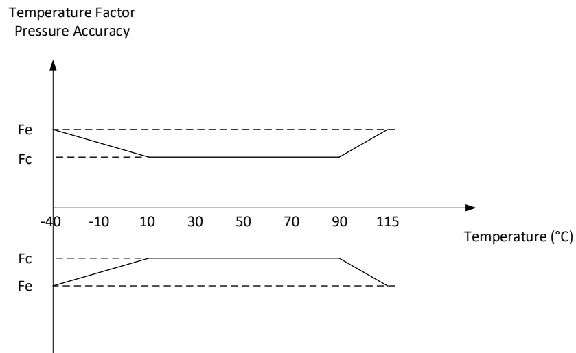
Figure 8: Pressure accuracy temperature factor (V temperature code)
