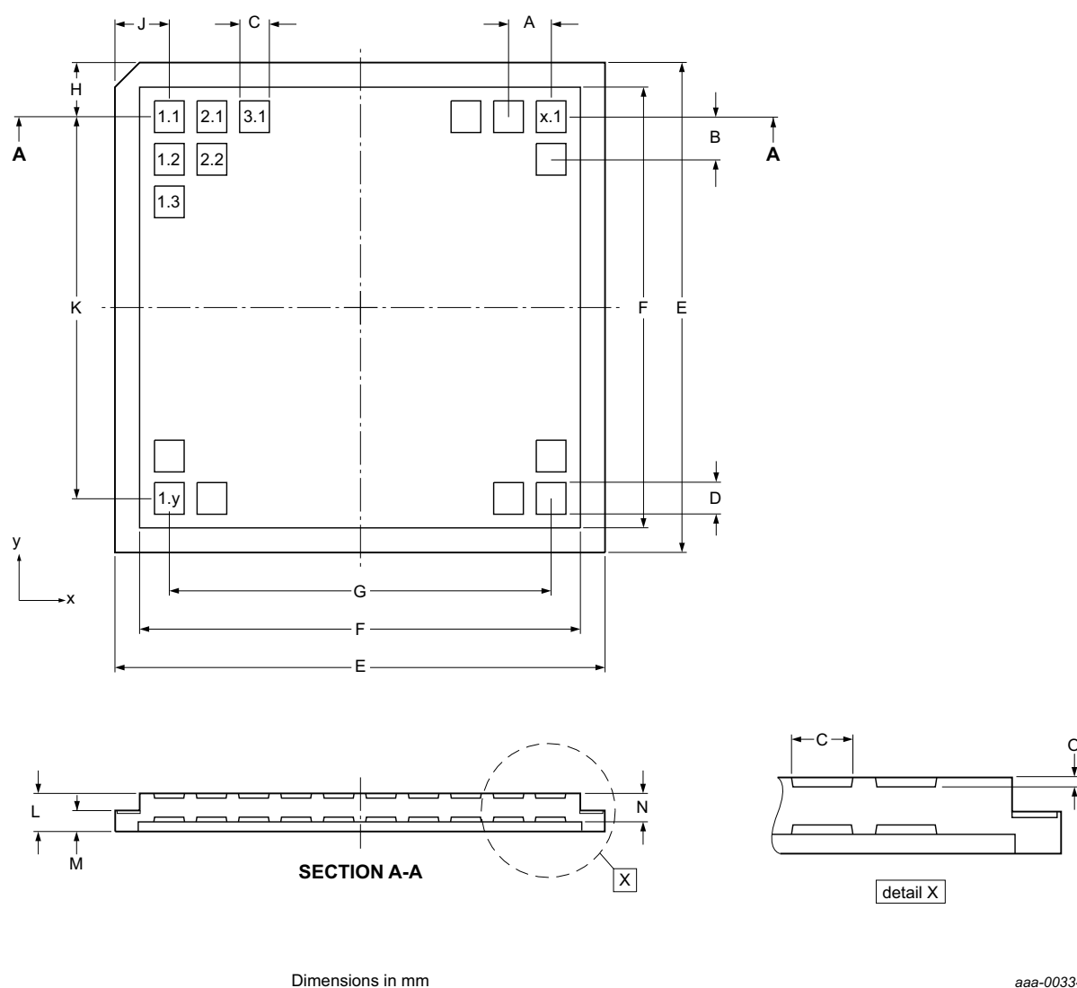
Fig 37. Tray details
