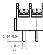
02 Circuit Board
