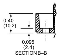
1, 3 & 5 Mount End
