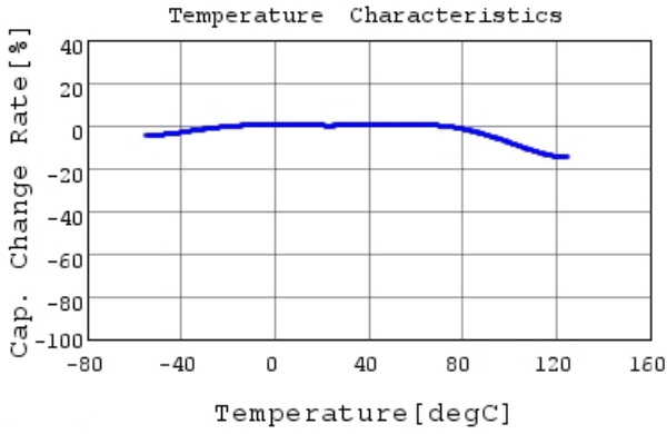
GRM188R71A105KA61 C-Temp. capchange, DC0.0V,
