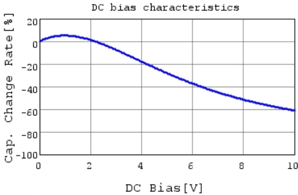
GRM188R71A105KA61 C-DC bias capchange, 25.0c
