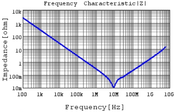
GRM188R71A105KA61 |Z| DCOV, 25degC
