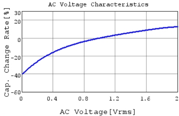
GRM188R71A105KA61 C-AC Voltage capchange, Dc
