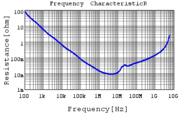
GRM188R71A105KA61 R DCOV, 25degC
