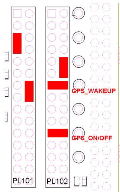
Figure 38. Settings for PL101 and PL102: internal host, cs1439b-A
