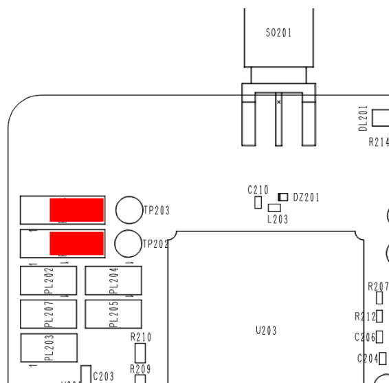
Figure 44. Jumpers in GSM to Trace configuration.
