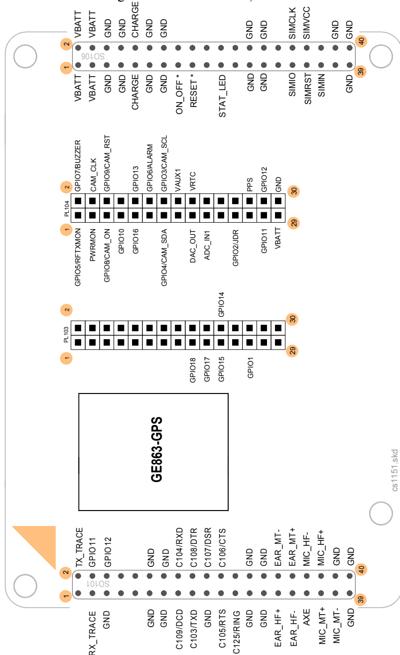
Figure 64: Position of GPIO ports on GE863-GPS interface
