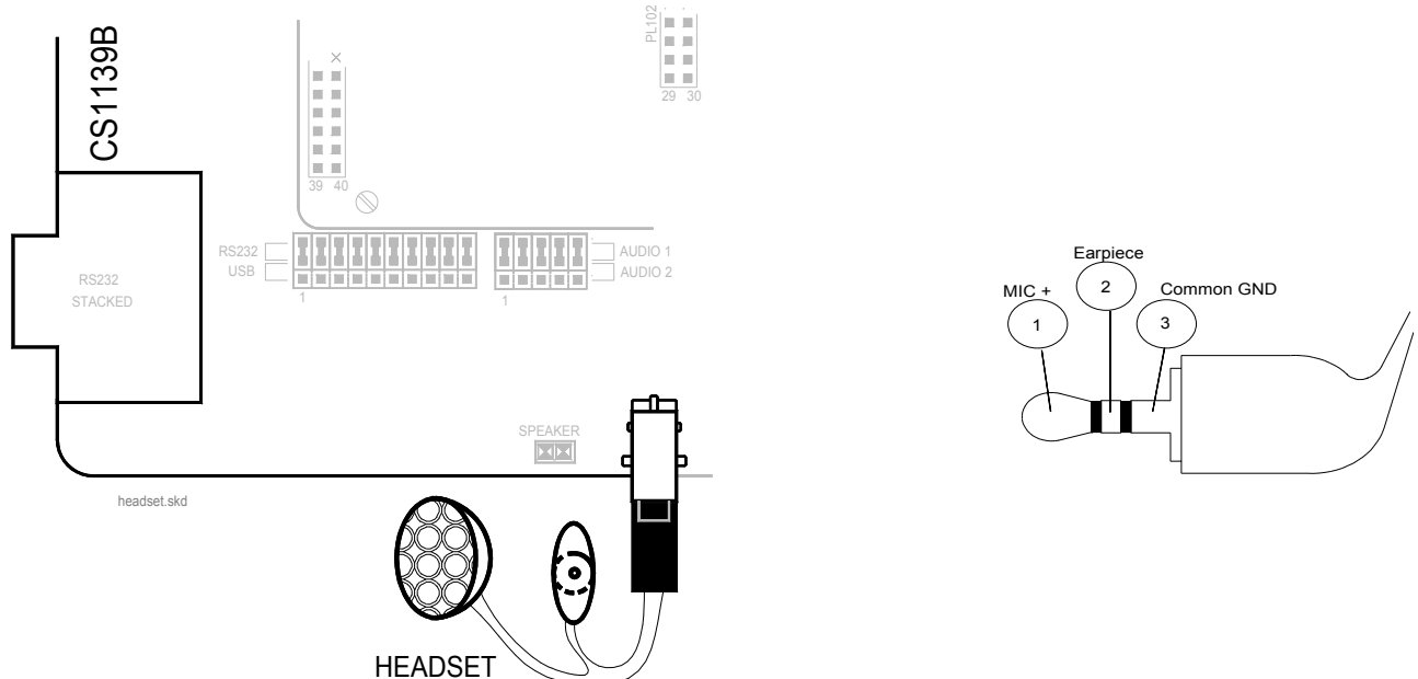
Figure 14: Headset insertion
