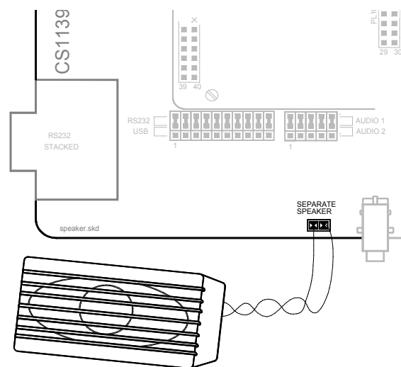
Figure 16: Speaker insertion
