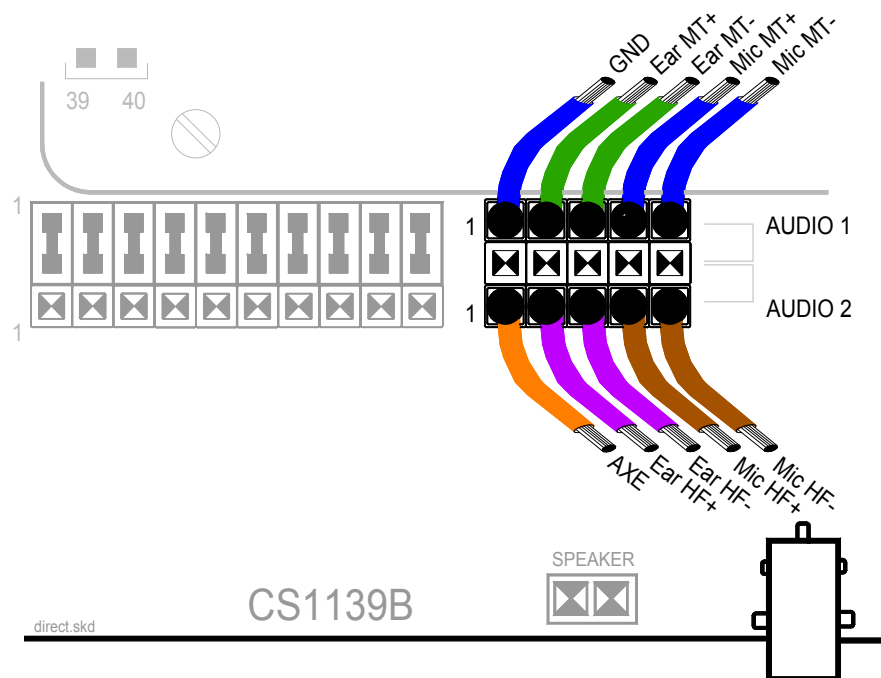
Figure 12: PL402 and PL404 Fully Differential audio lines.
