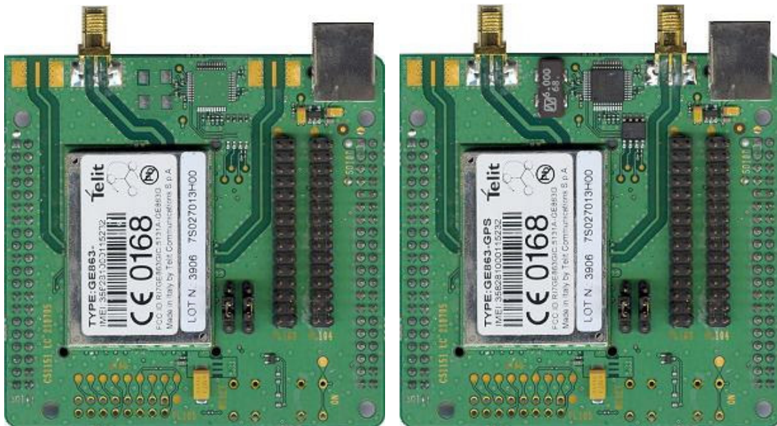
Figure 24. GE863 Interface Boards: GE863-QUAD or GE863-SIM (at left) and GE863-GPS (at right)
