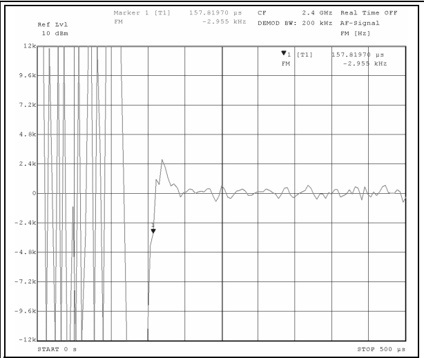
Figure 14. Settling time (final frequency=2.4 GHz; F_{PFD}=400\text{ kHz} ; I_{CP}=2.5\text{ mA} )
