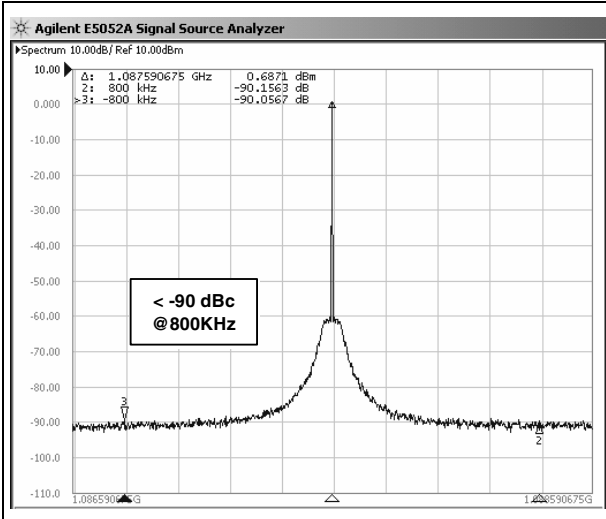
Figure 13. PFD frequency spurs (div. by 4 output; F_{PFD}=800\text{ kHz} )
