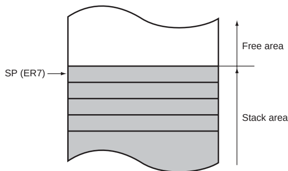
Figure 2.8 Stack
