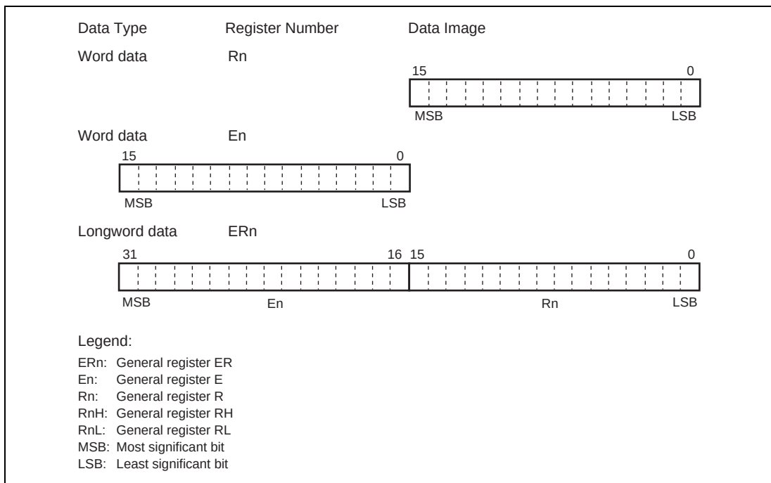
Figure 2.9 General Register Data Formats (2)
