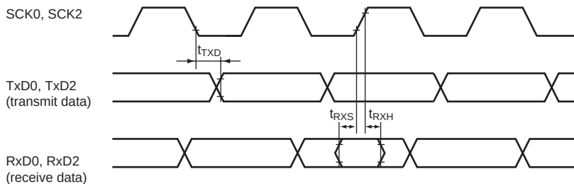
Figure 22.16 SCI Input/Output Timing (Clock Synchronous Mode)
