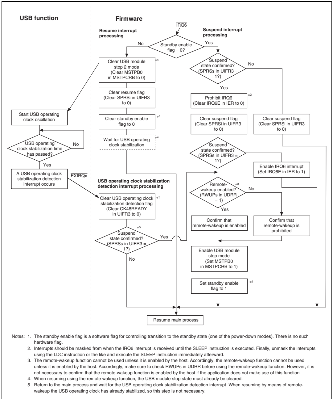
Figure 14.8 Example Flowchart of Suspend and Resume Interrupt Processing
