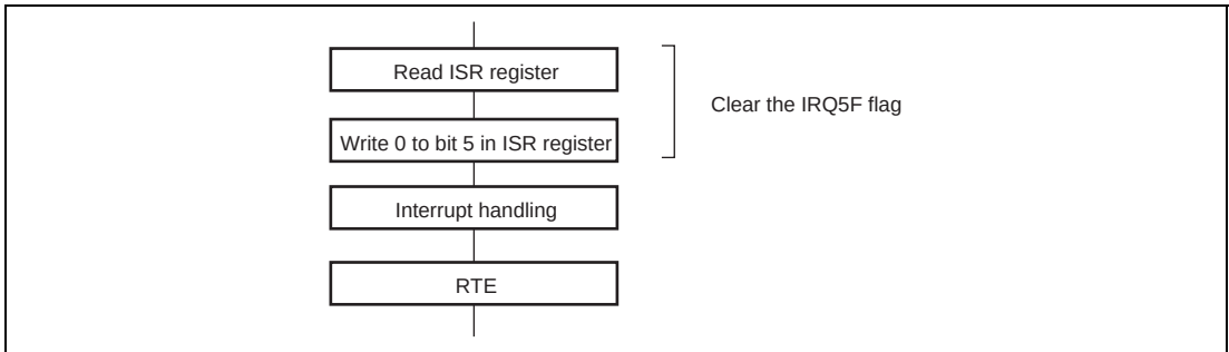
Figure 11.6 Example of RTC Interrupt Handling Routine
