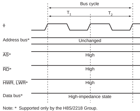
Figure 6.7 Pin States during On-Chip Peripheral Module Access
