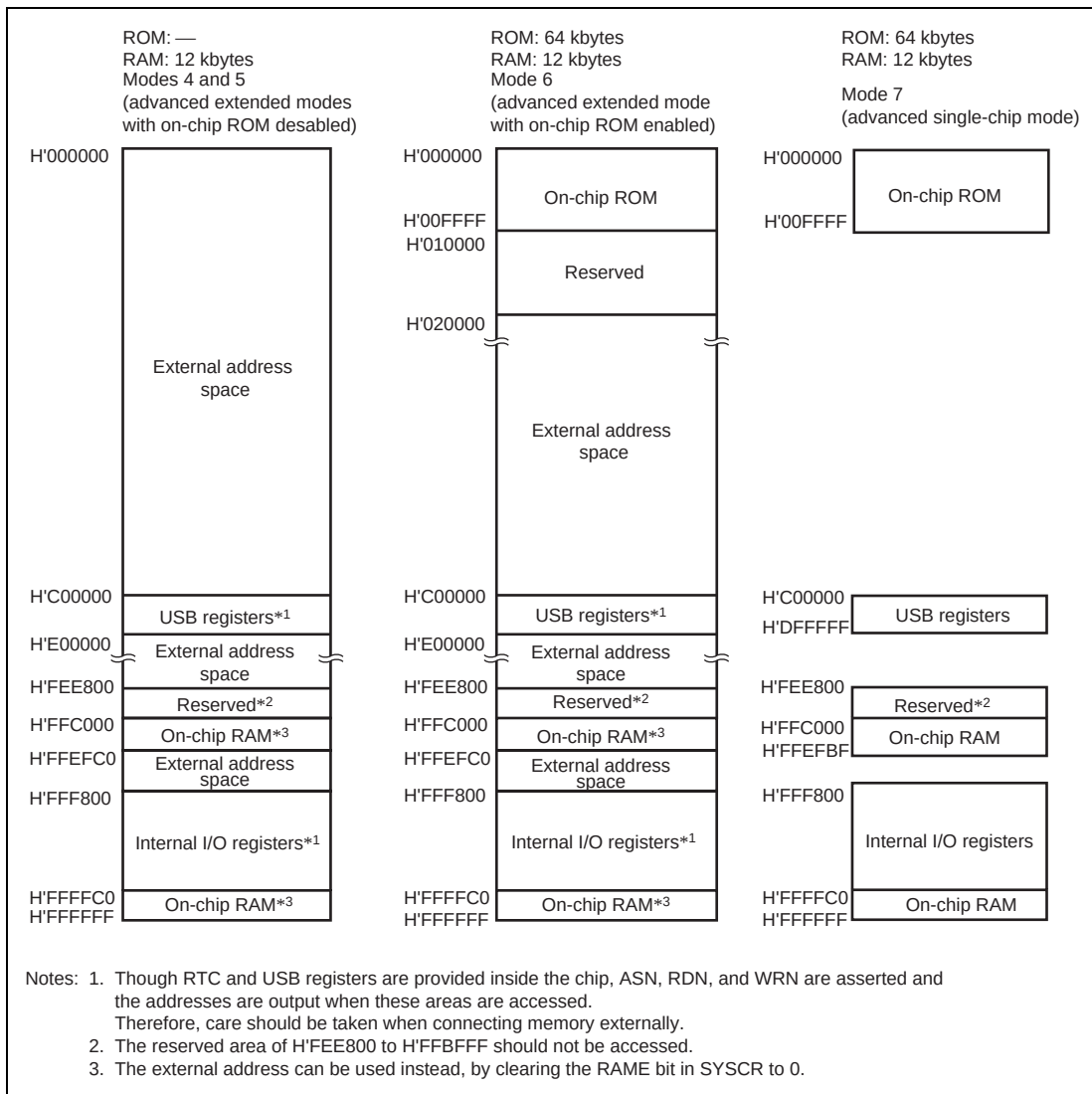
Figure 3.2 Memory Map in Each Operating Mode for HD64F2217CU
