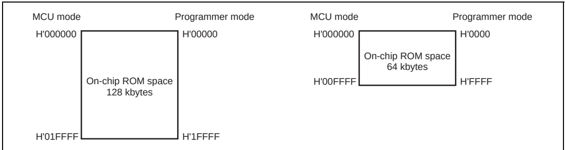
Figure 17.15 Memory Map in Programmer Mode
