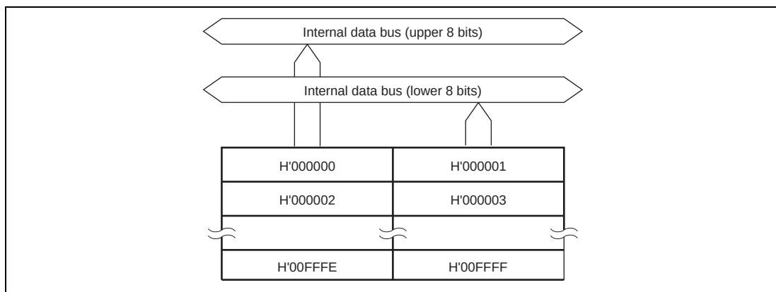
Figure 18.1 Block Diagram of On-Chip Masked ROM (64 kbytes)
