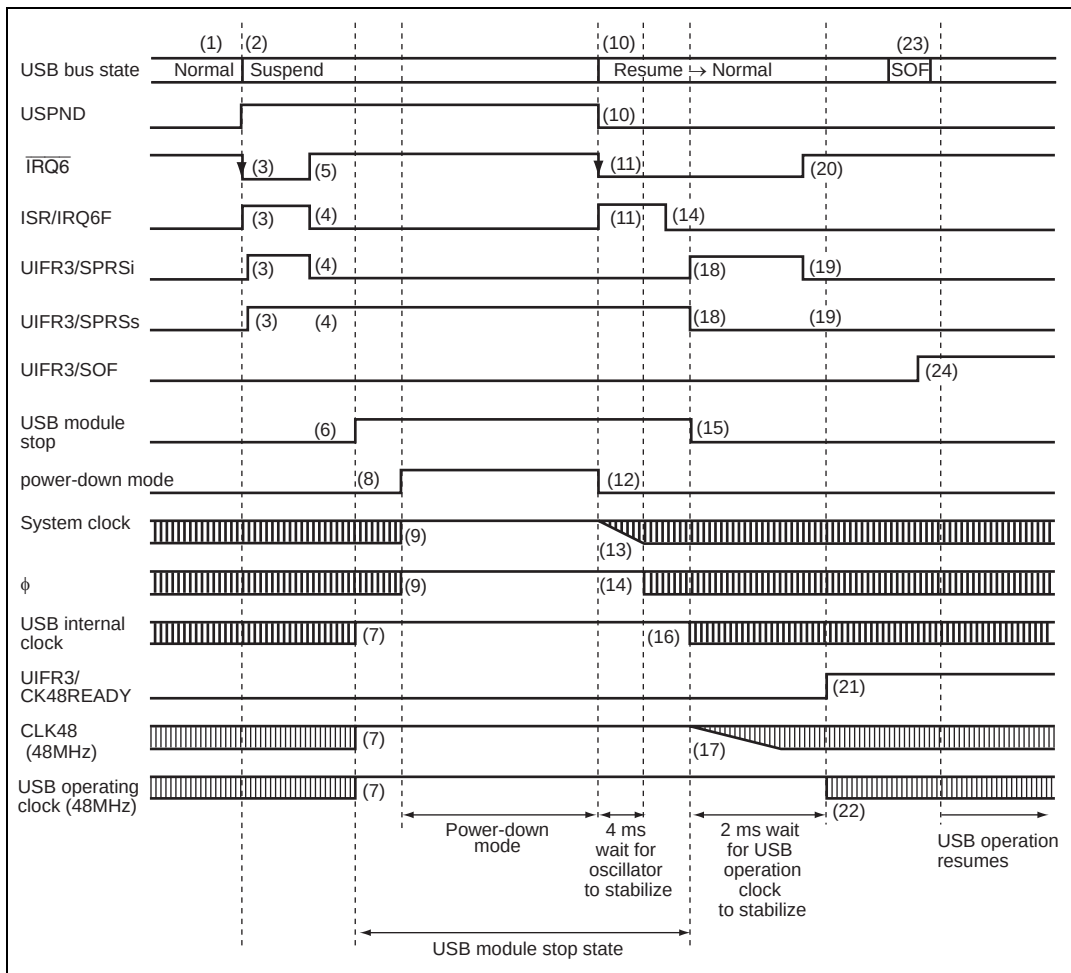
Figure 14.29 Timing Chart
