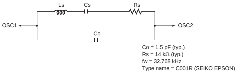
Figure 19.7 Equivalence Circuit for 32.768-kHz Oscillator
