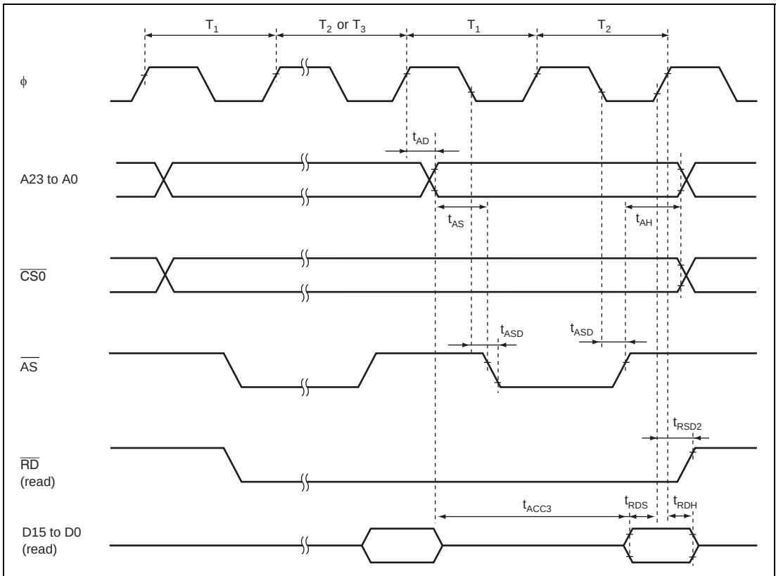
Figure 22.10 Burst ROM Access Timing (Two-State Access)
