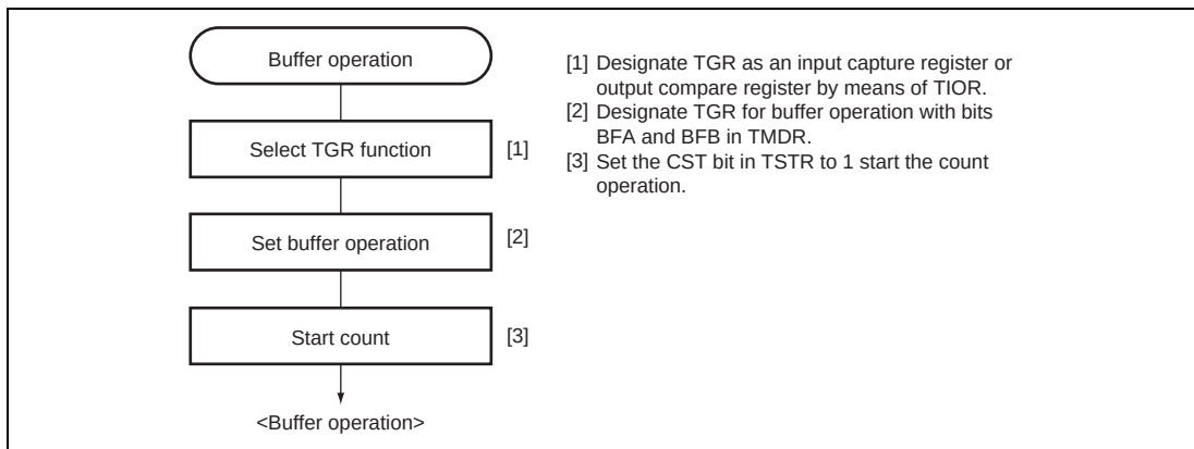
Figure 9.18 Example of Buffer Operation Setting Procedure
