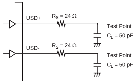
Figure 22.22 Test Load Circuit
