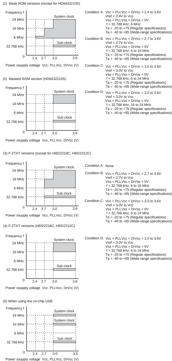
Figure 22.1 Power Supply Voltage and Operating Ranges
