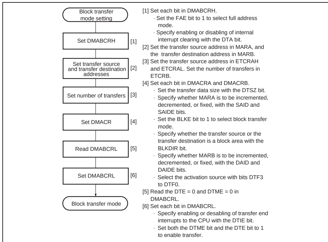
Figure 7.13 Example of Block Transfer Mode Setting Procedure
