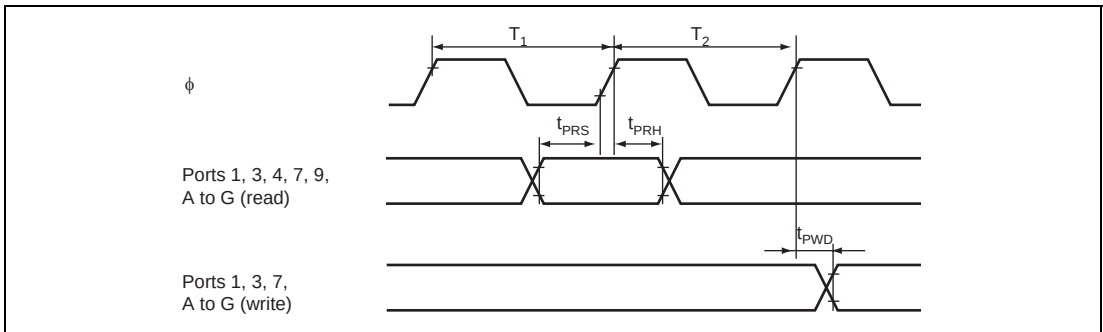
Figure 22.12 I/O Port Input/Output Timing
