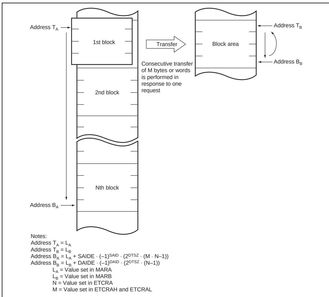
Figure 7.10 Operation in Block Transfer Mode (BLKDIR = 0)
