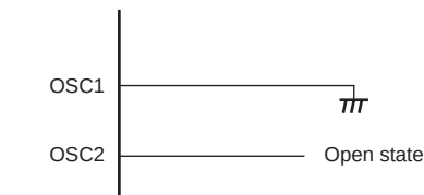
Figure 19.8 Pin Handling when Subclock Not Required
