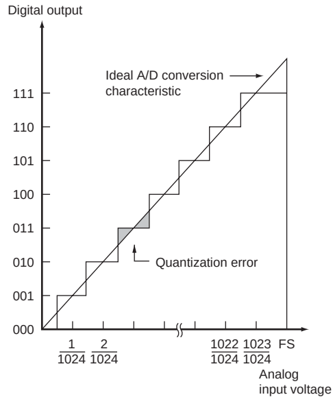
Figure 15.7 A/D Conversion Precision Definitions (1)
