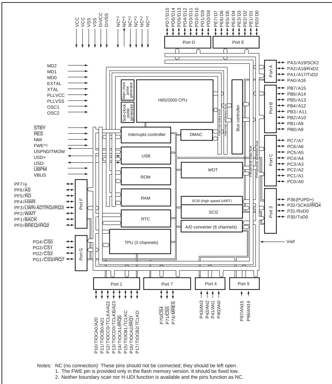
Figure 1.2 Internal Block Diagram of HD6432217
