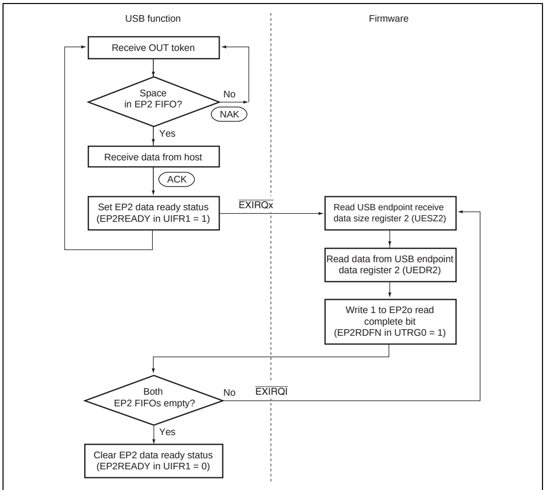
Figure 14.19 EP2 Bulk-Out Transfer Operation
