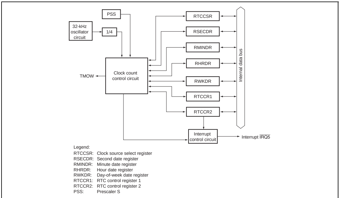
Figure 11.1 Block Diagram of RTC
