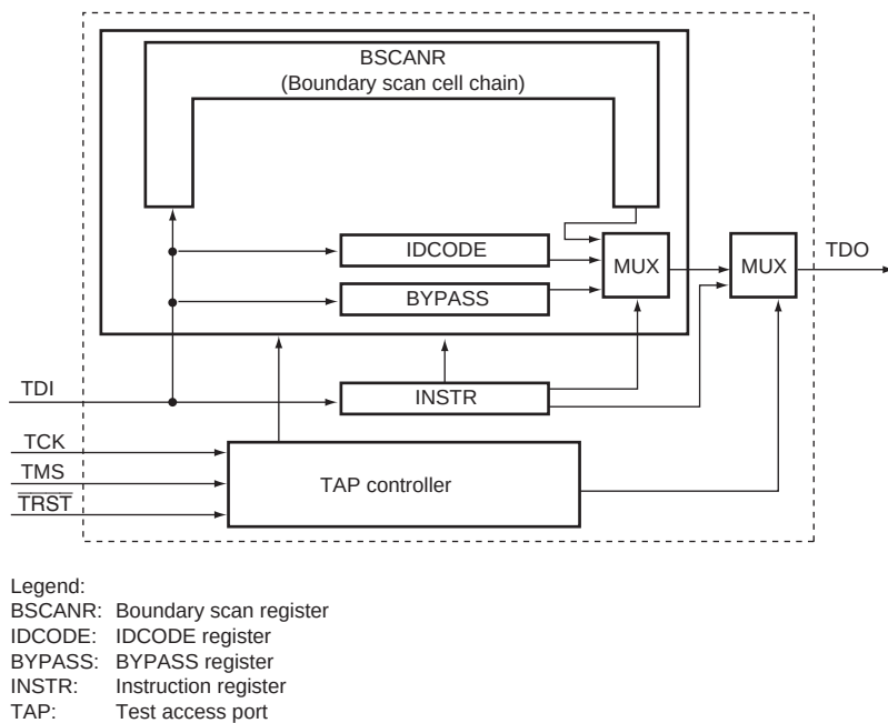
Figure 13.1 Block Diagram of Boundary Scan Function
