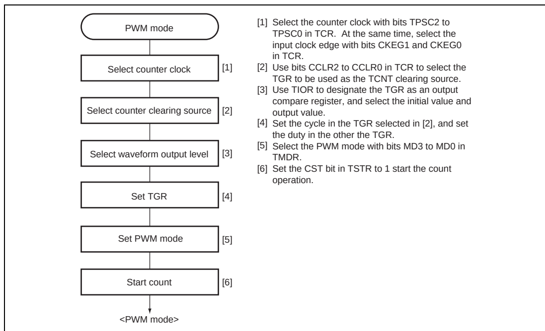
Figure 9.21 Example of PWM Mode Setting Procedure
