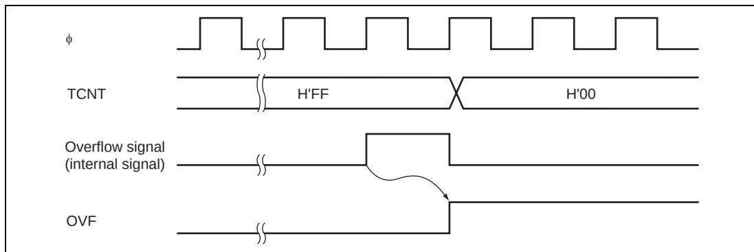
Figure 10.5 Timing of OVF Setting
