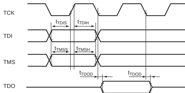
Figure 22.20 Boundary Scan Data Transmission Timing
