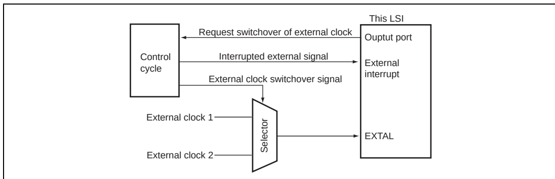
Figure 19.11 Example of External Clock Switching Circuit
