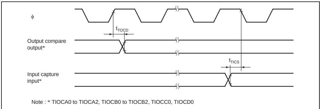
Figure 22.13 TPU Input/Output Timing
