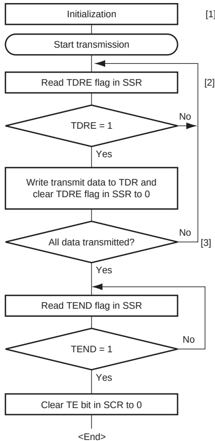
Figure 12.20 Sample Serial Data Transmission Flowchart
