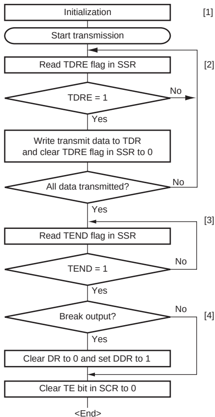
Figure 12.10 Sample Serial Data Transmission Flowchart
