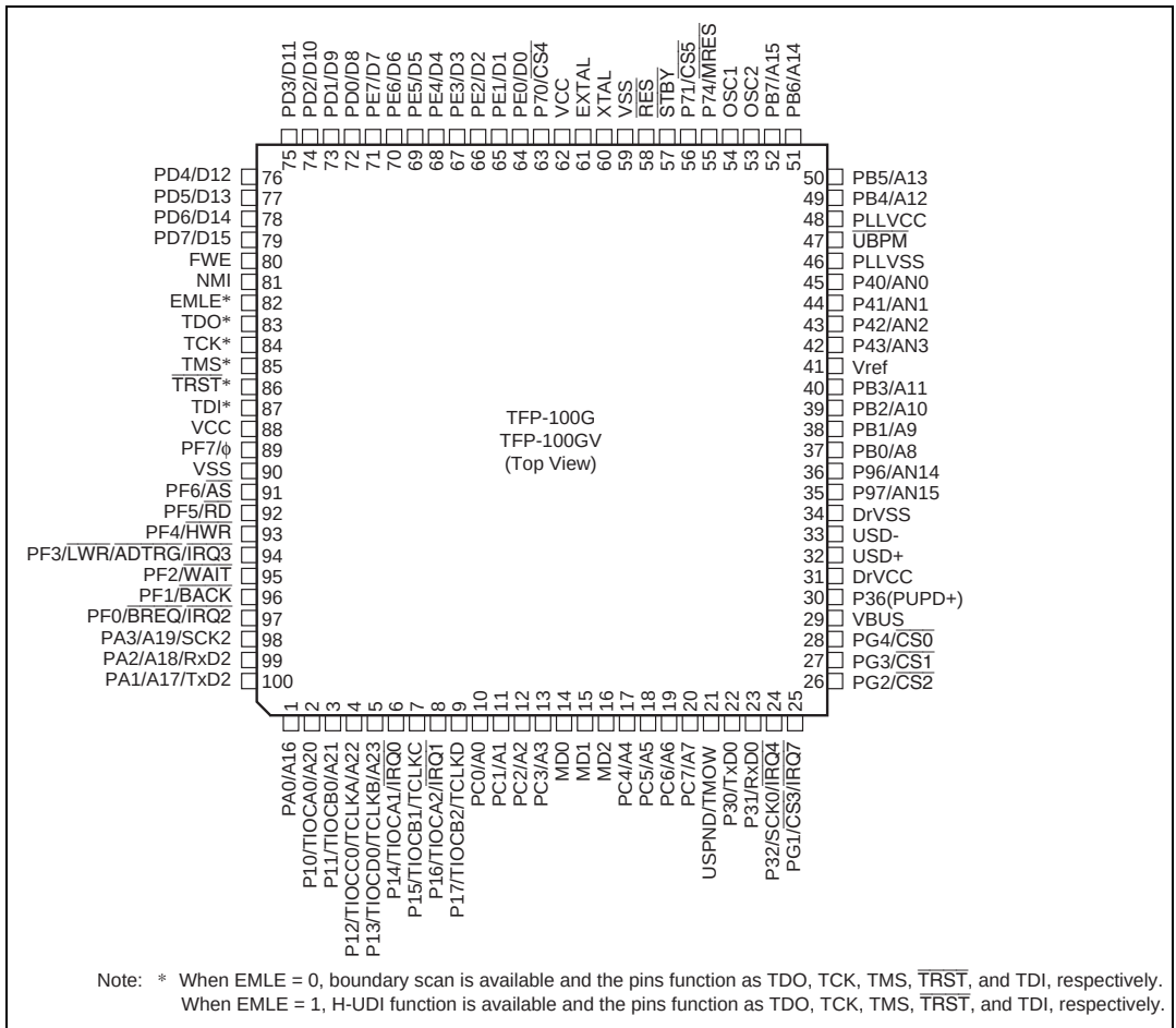
Figure 1.5 Pin Arrangements of HD64F2218, HD64F2218U, HD64F2218CU and HD64F2217CU (TFP-100G, TFP-100GV)
