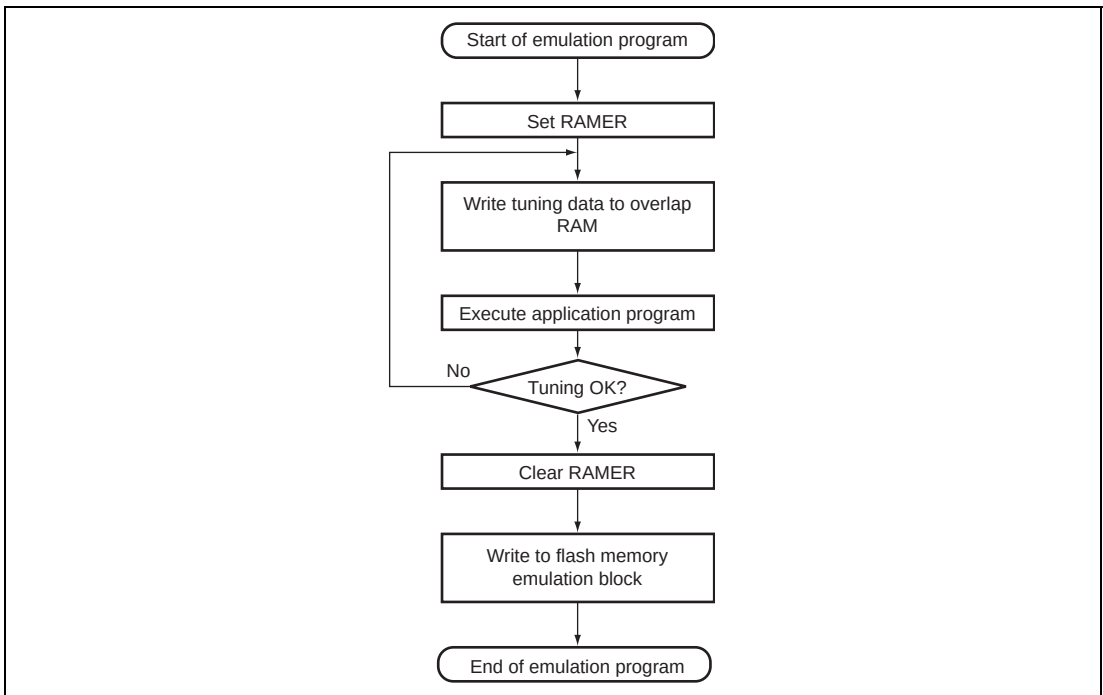
Figure 17.11 Flowchart for Flash Memory Emulation in RAM
