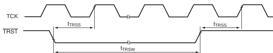
Figure 22.19 Boundary Scan \overline{\text{TRST}} Input Timing (At Reset Hold)
