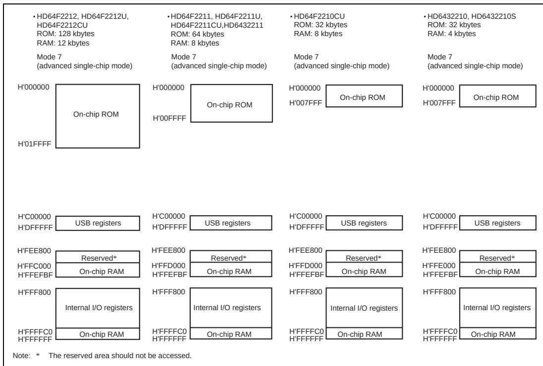
Figure 3.4 Memory Map in Each Operating Mode for HD64F2212, HD64F2212U, HD64F2212CU, HD64F2211, HD64F2211U, HD64F2211CU, HD64F2210CU, HD6432211, HD6432210 and HD6432210S
