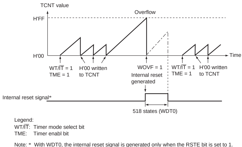
Figure 10.2 Operation in Watchdog Timer Mode
