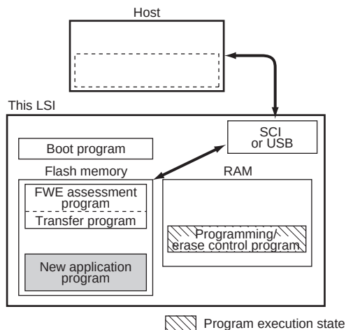
Figure 17.4 User Program Mode (Sample)
