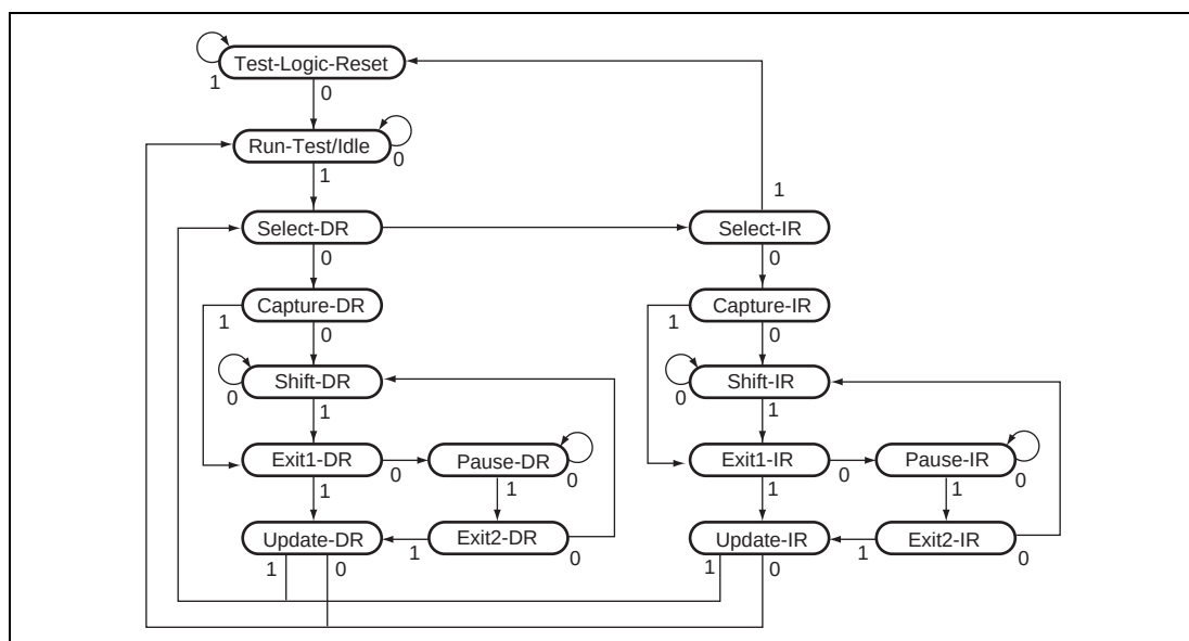
Figure 13.3 TAP Controller Status Transition
