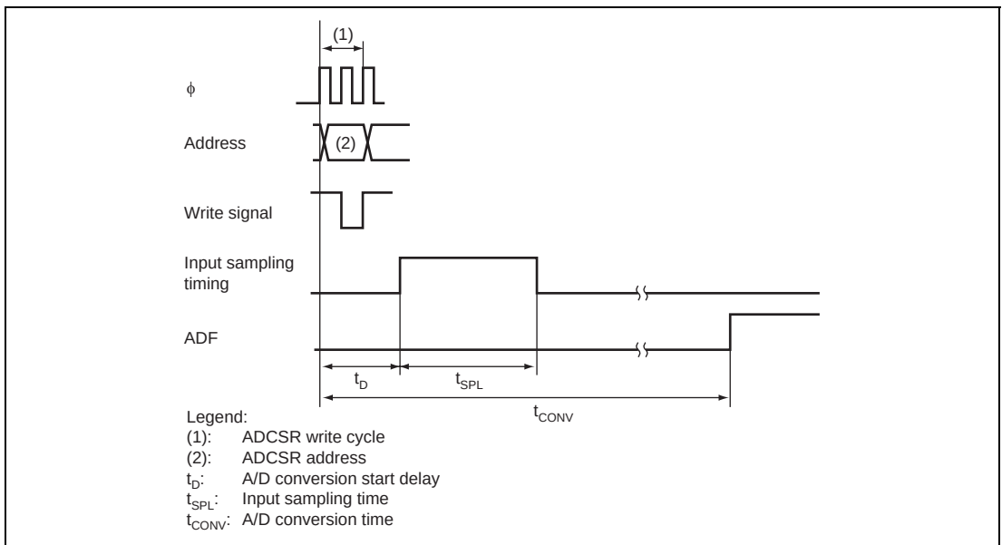
Figure 15.5 A/D Conversion Timing
