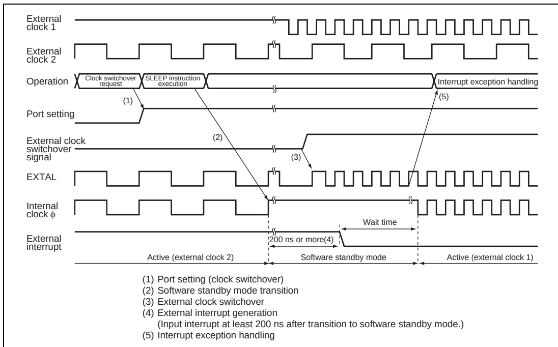
Figure 19.12 Example of External Clock Switchover Timing
