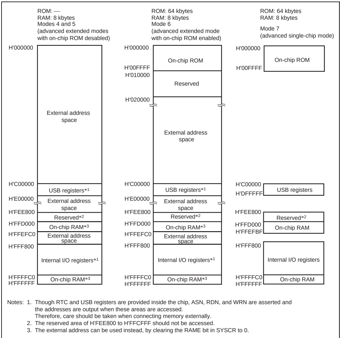
Figure 3.3 Memory Map in Each Operating Mode for HD6432217
