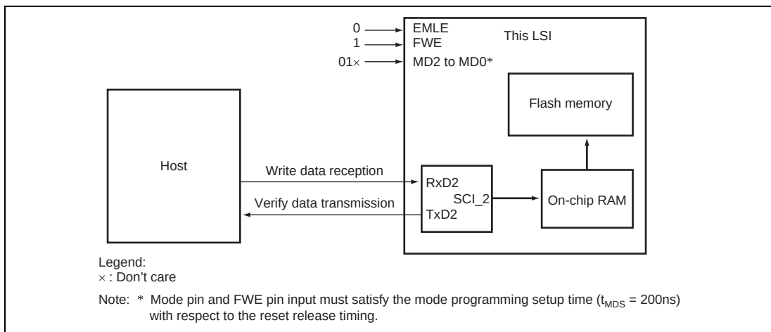
Figure 17.8 System Configuration in SCI Boot Mode
