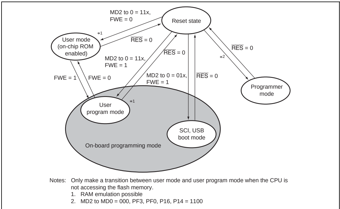
Figure 17.2 Flash Memory State Transitions
