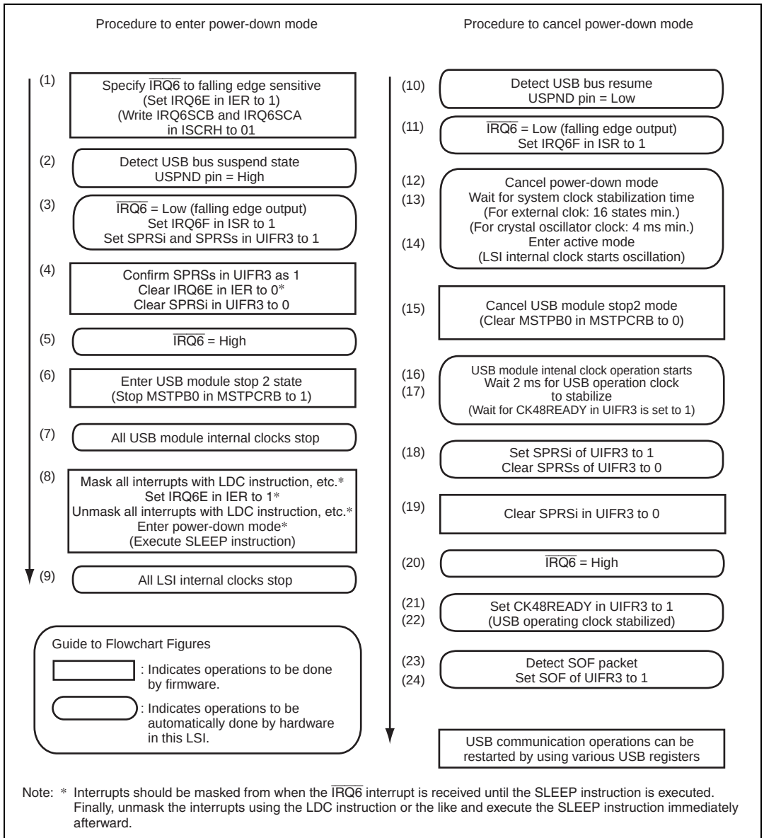
Figure 14.28 Flowchart
