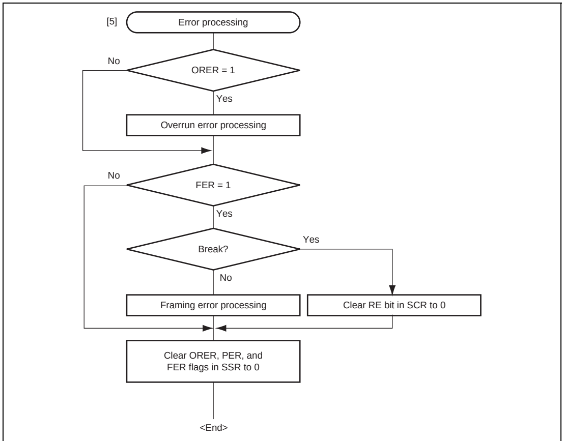
Figure 12.16 Sample Multiprocessor Serial Data Reception Flowchart (2)
