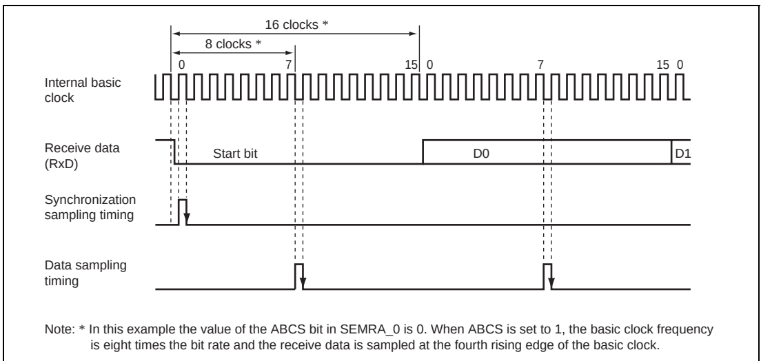
Figure 12.6 Receive Data Sampling Timing in Asynchronous Mode
