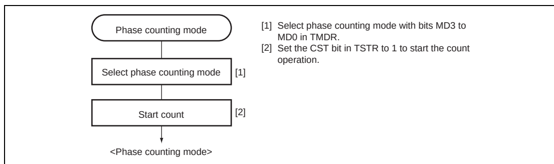
Figure 9.25 Example of Phase Counting Mode Setting Procedure
