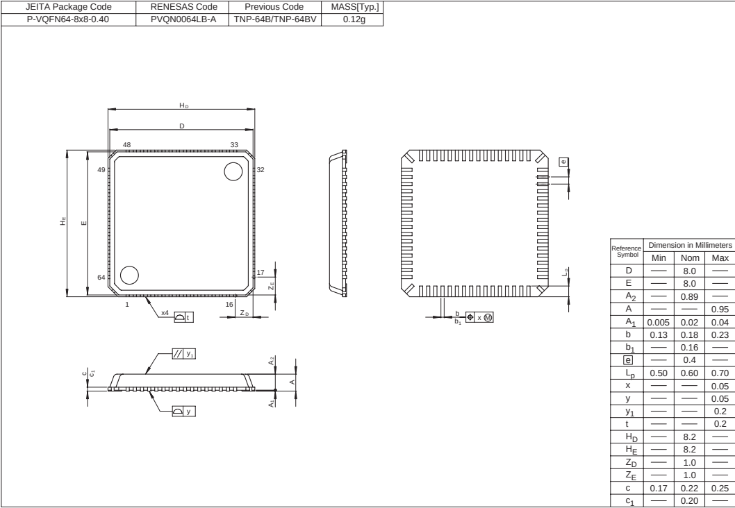
Figure C.4 TNP-64B and TNP-64BV Package Dimensions
