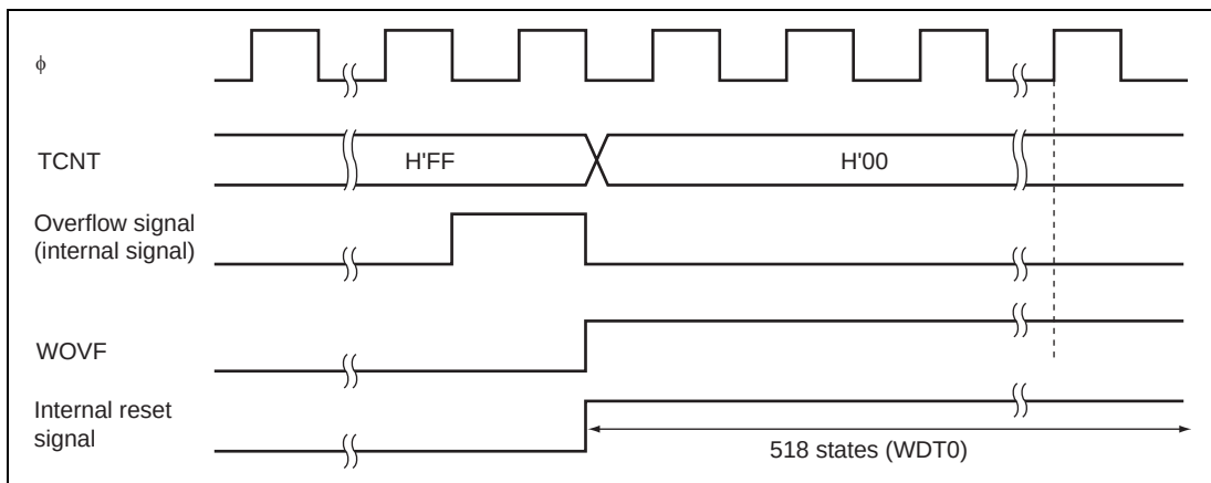
Figure 10.3 Timing of WOFV Setting
