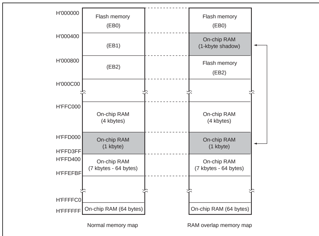
Figure 17.12 Example of RAM Overlap Operation
