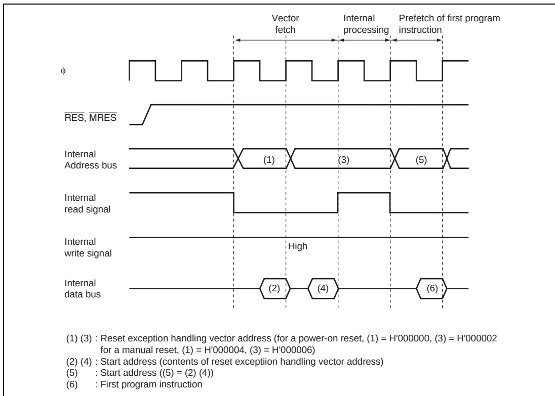
Figure 4.2 Reset Sequence (Modes 6 and 7)
