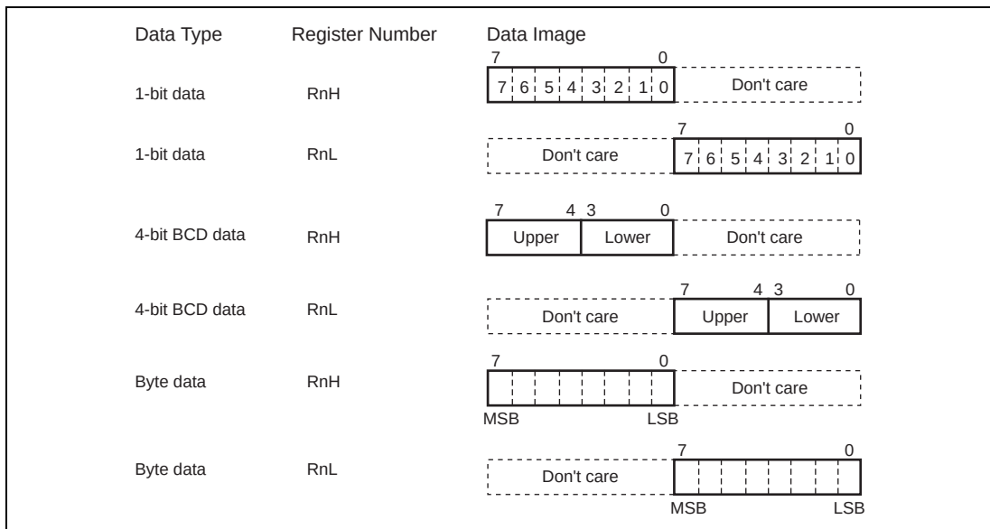
Figure 2.9 General Register Data Formats (1)
