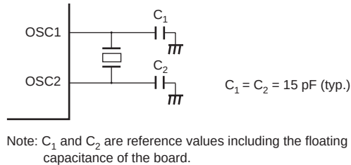
Figure 19.6 Example Connection of 32.768-kHz Quartz Oscillator
