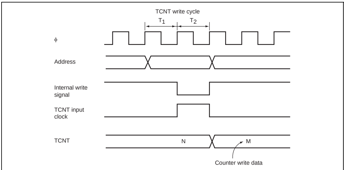
Figure 10.8 Contention between TCNT Write and Increment
