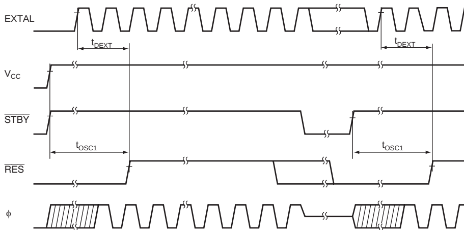
Figure 22.4 Oscillation Stabilization Timing
