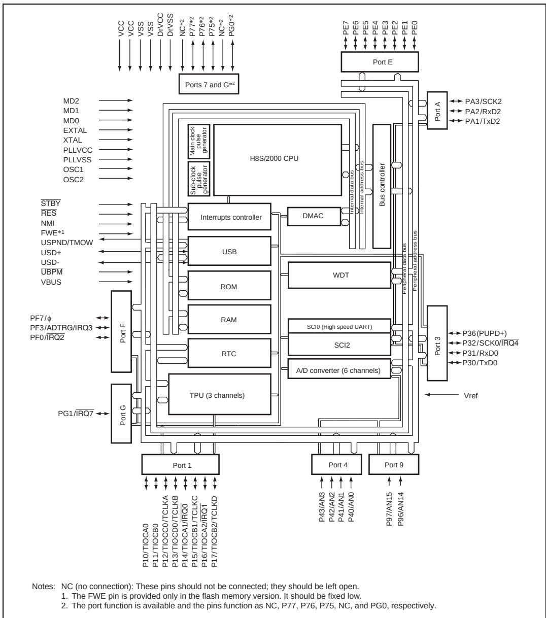
Figure 1.4 Internal Block Diagram of HD6432211, HD6432210 and HD6432210S
