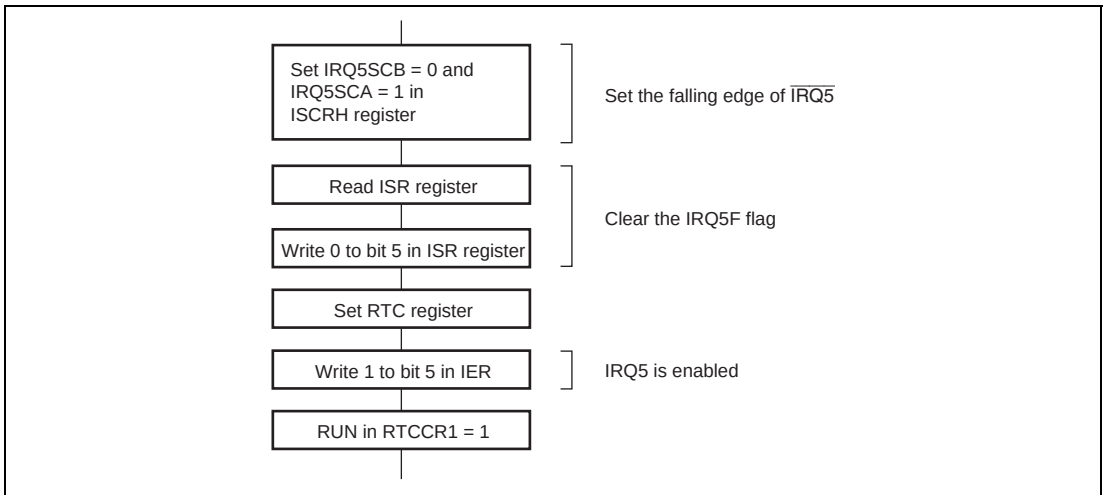
Figure 11.5 Initializing Procedure in Using RTC Interrupt
