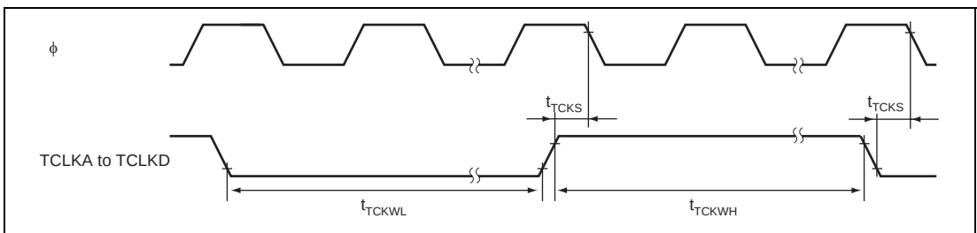
Figure 22.14 TPU Clock Input Timing
