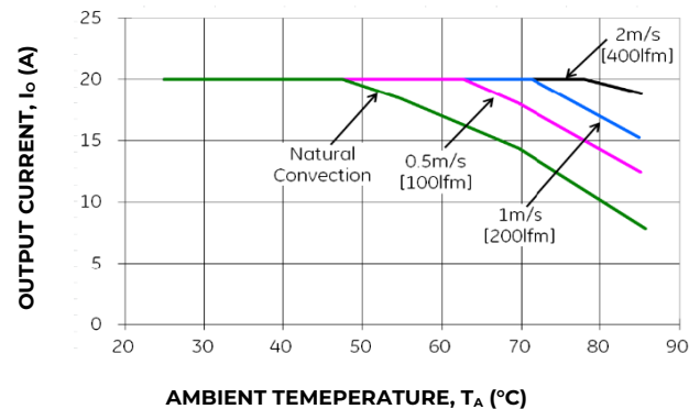
Figure 19. Output Current Derating for the Open Frame Module; Airflow in the Transverse Direction from V_{out}(-) to V_{out}(+) ; V_{IN}=24V
