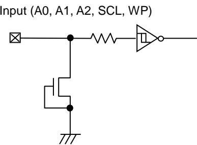
Figure 50. Input Pin Circuit Diagram
