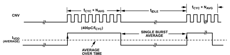
Figure 76. I_{DD} vs. Burst Conversions in Burst Averaging Mode
