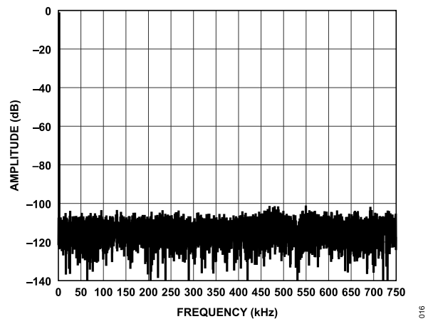
Figure 16. Fast Fourier Transform (FFT), f_S = 1.5\text{ MSPS} , f_{IN} = 1\text{ kHz}
