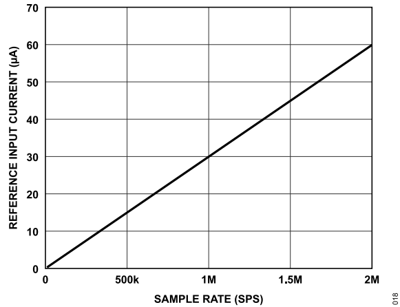
Figure 18. Reference Input Current vs. Sample Rate
