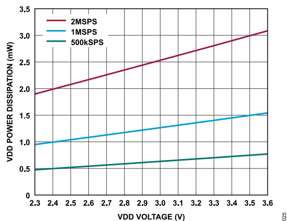
Figure 25. VDD Power Dissipation vs. VDD Voltage
