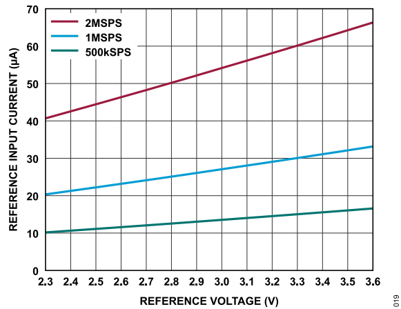
Figure 19. Reference Input Current vs. Reference Voltage
