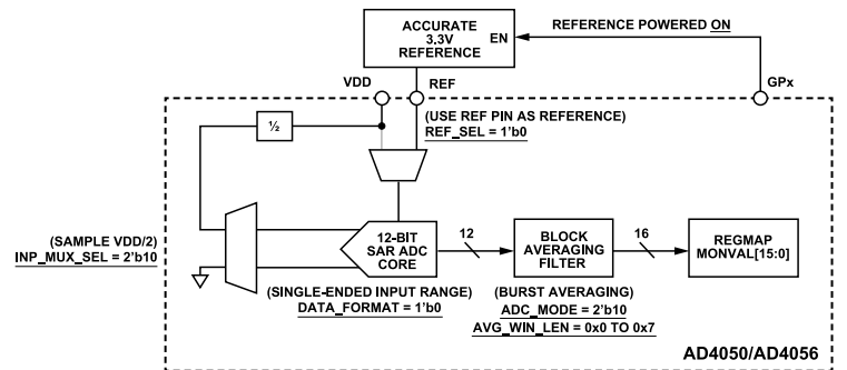
Figure 73. MON_VAL Calculation Configuration
