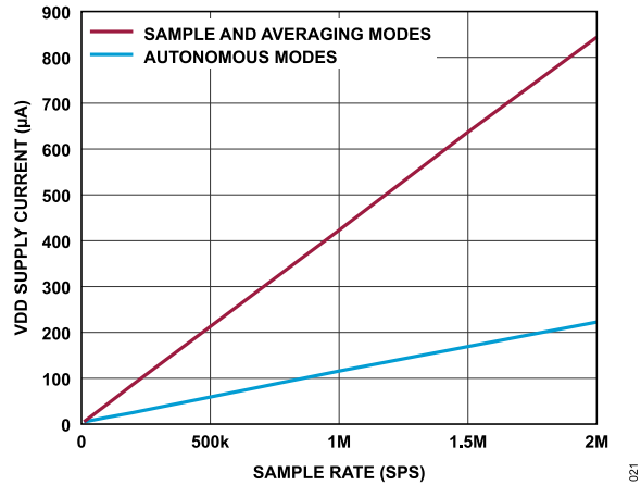
Figure 21. VDD Supply Current vs. Sample Rate
