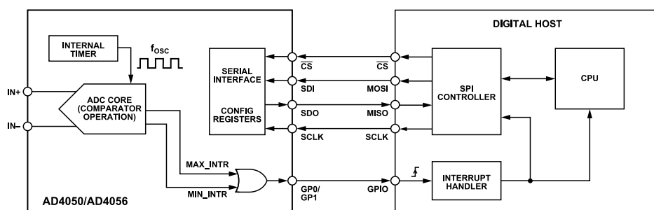
Figure 60. Autonomous Mode Example Connection Diagram
