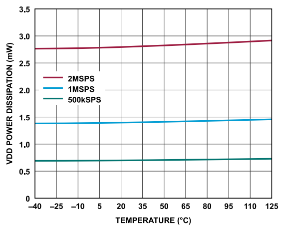
Figure 26. VDD Power Dissipation vs. Temperature
