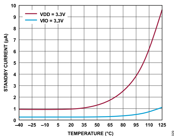
Figure 29. Standby Current vs. Temperature
