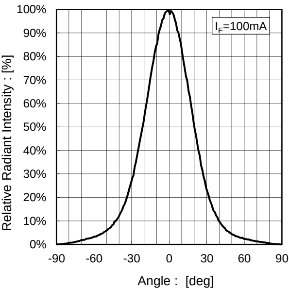
Fig.6 Radiant Intensity
