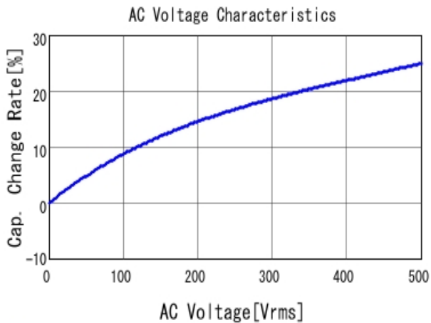
■ DE1B3RB471KJ4BR01F C-AC Voltage capchange, DC0V, 20.0
