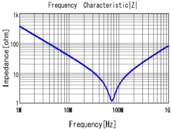
■ DE1B3RB471KJ4BR01F |Z| DC0V, 20degC
