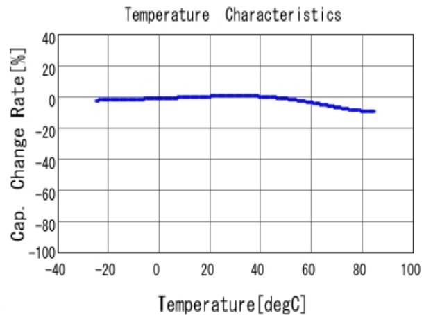
■ DE1B3RB471KJ4BR01F C-Temp. capchange, DC0V, AC1Vrms
