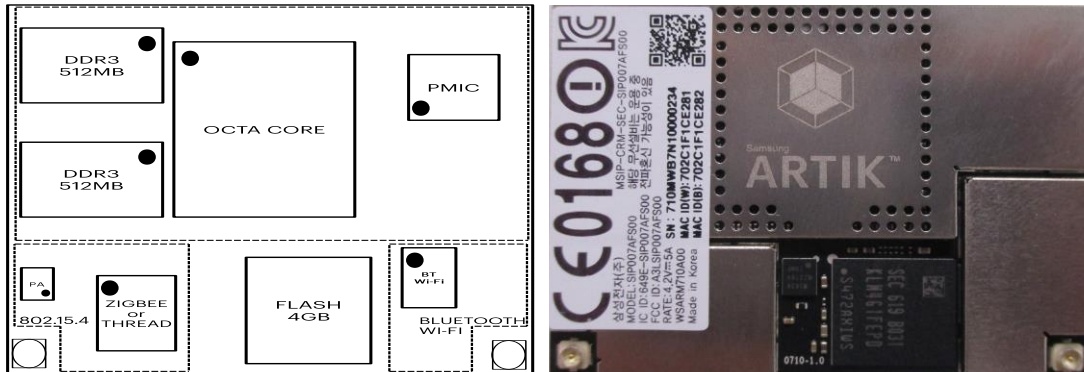
Figure 2. ARTIK 710 Module Component Placement - Top View
