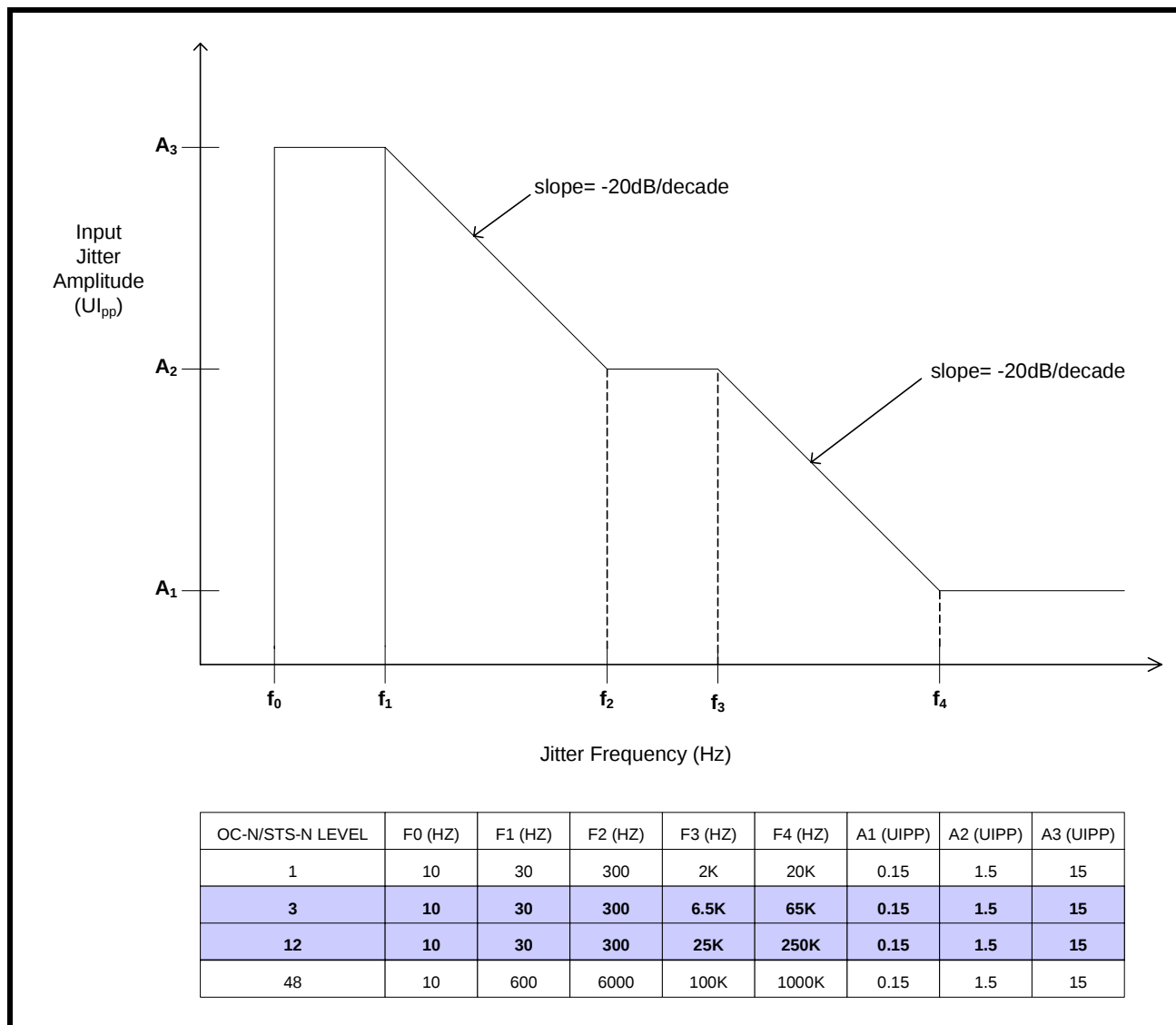
FIGURE 22. JITTER TOLERANCE MASK
