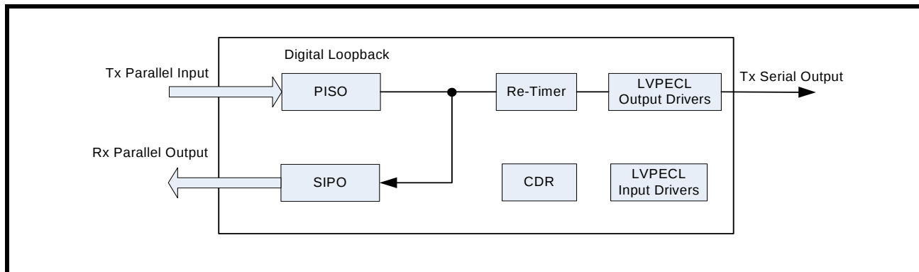
FIGURE 17. DIGITAL LOCAL LOOPBACK
