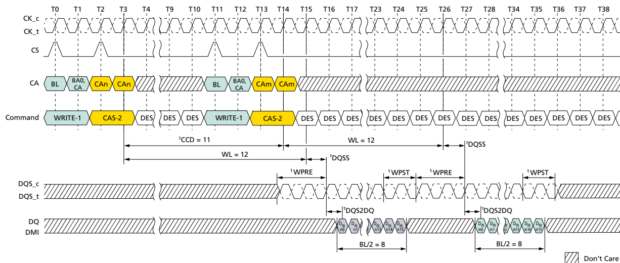
Figure 64: Consecutive WRITE: t_{CCD} = \text{MIN} + 3, 1.5nCK Postamble
