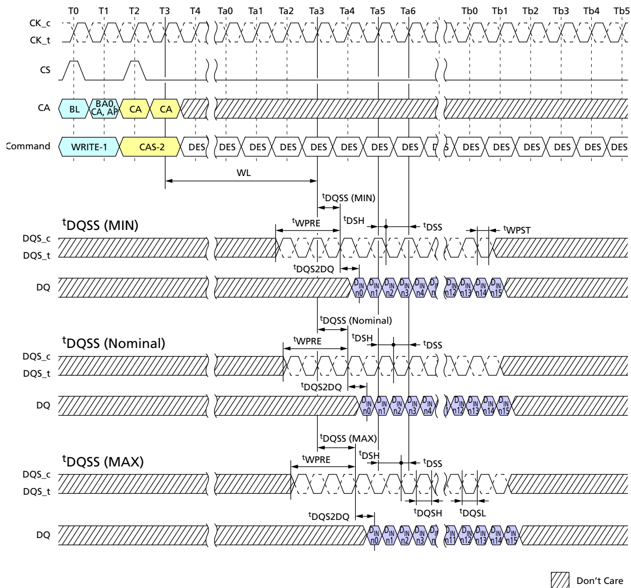
Figure 32: Write Timing
