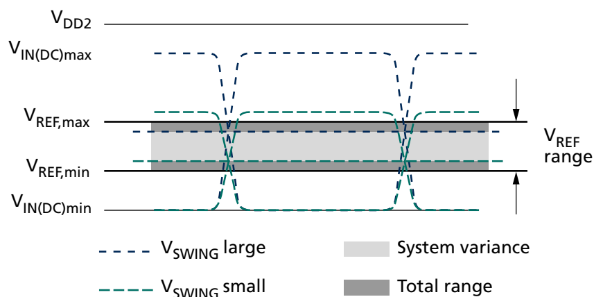
Figure 102: V_{REF} Operating Range ( V_{REF,max} , V_{REF,min} )
