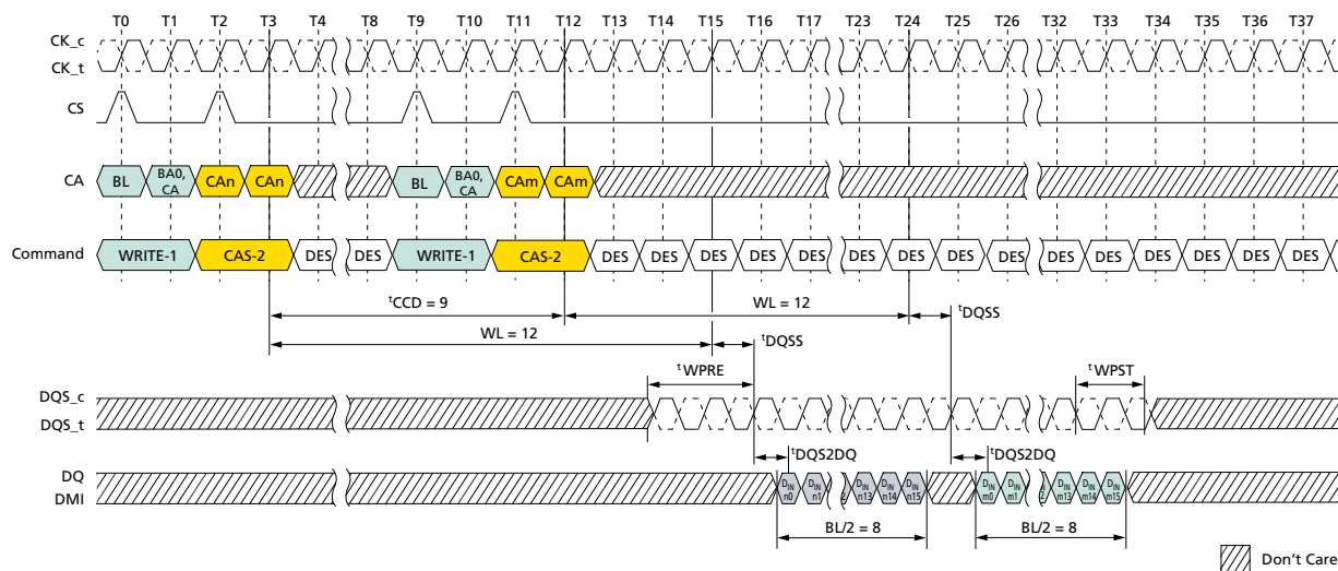
Figure 60: Consecutive WRITE: t_{CCD} = \text{MIN} + 1, 1.5nCK Postamble
