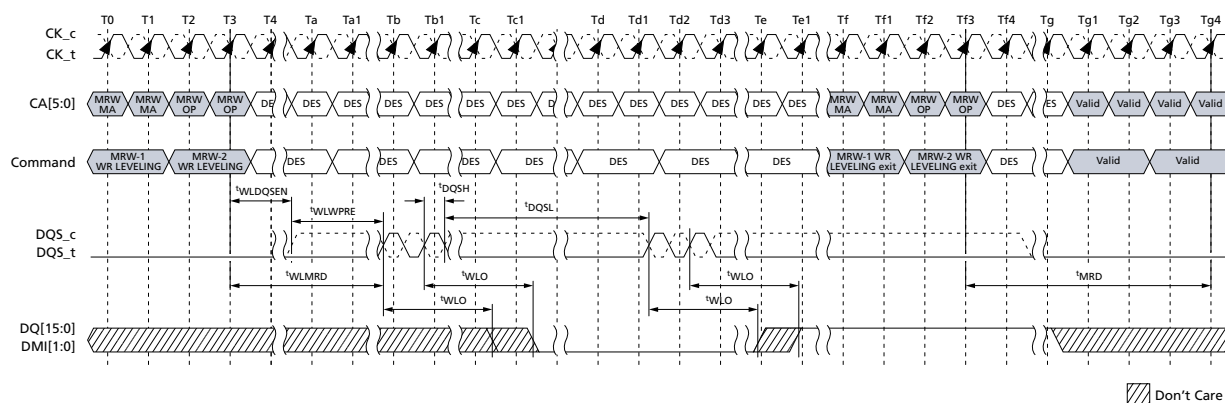
Figure 120: Write Leveling Timing – t_{DQSL}(\text{MAX})
