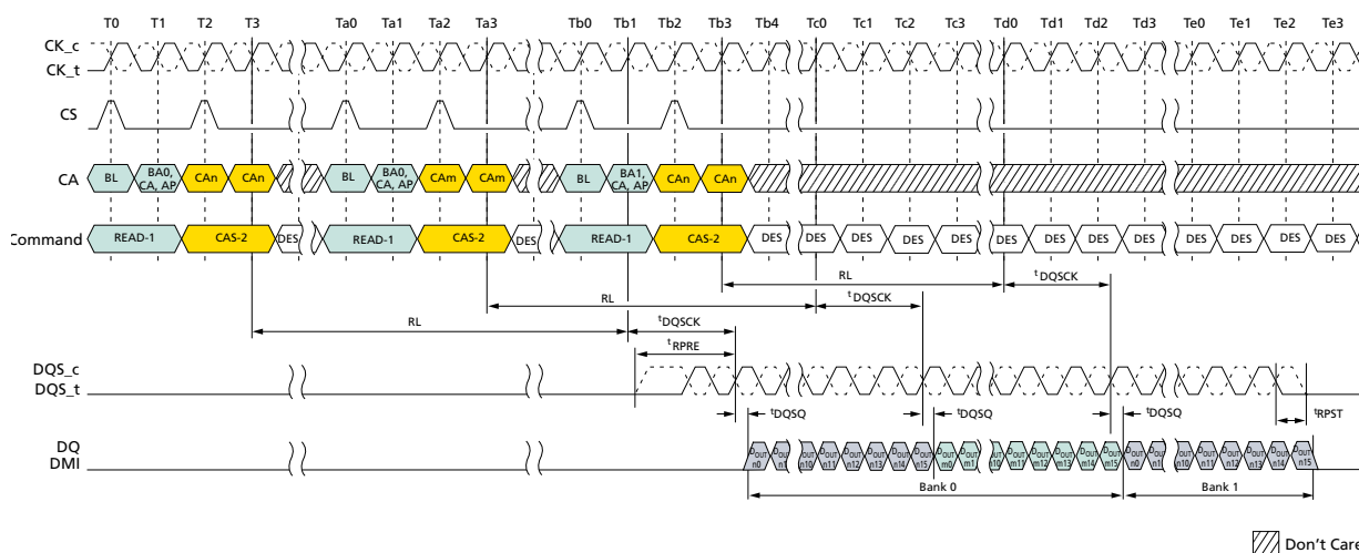
Figure 24: Seamless Burst Read
