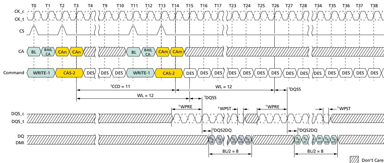
Figure 63: Consecutive WRITE: t_{CCD} = \text{MIN} + 3, 0.5nCK Postamble
