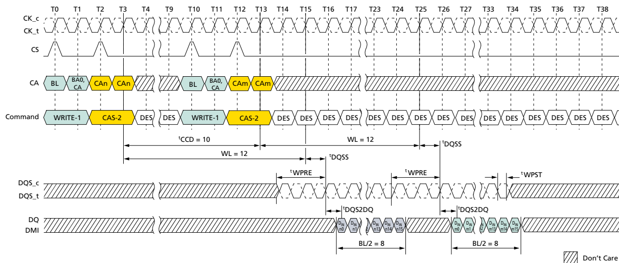
Figure 61: Consecutive WRITE: t_{CCD} = \text{MIN} + 2, 0.5n\text{CK} Postamble
