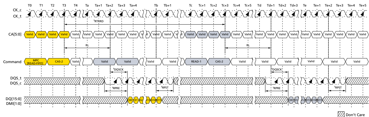
Figure 126: READ-FIFO – t_{RPRE} = \text{Toggle} , t_{RPST} = 1.5nCK
