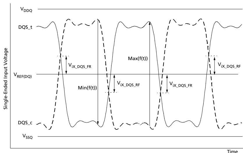
Figure 162: V_{IX} Definition (DQS)
