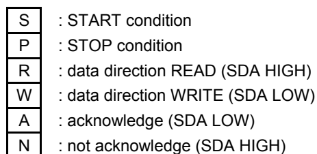
Figure 7. Read/Write Protocol
