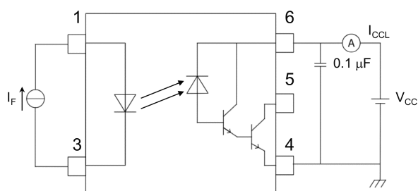
Fig. 12.1.3 I_{CCL} Test Circuit
