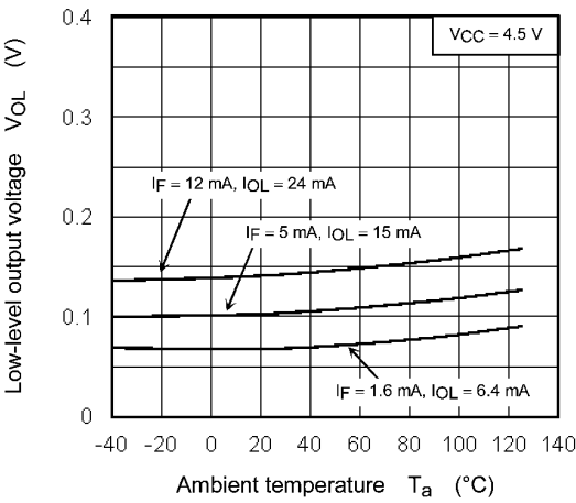
Fig. 12.2.6 V_{OL} - T_a
