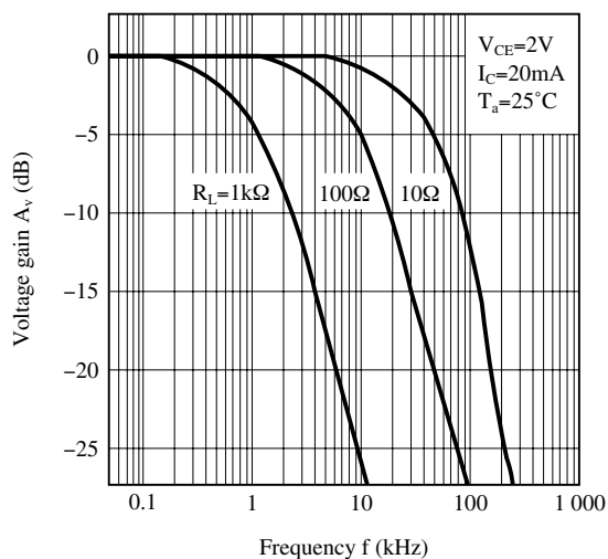
Fig.14 Frequency Response
