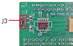
Fig 2: J3 Header
