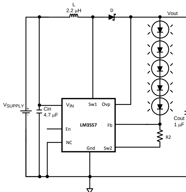
Figure 1. Backlight Configuration
