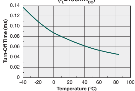
Typical Turn-Off Time vs. Temperature ( I_L=150\text{mA}_{DC} )
