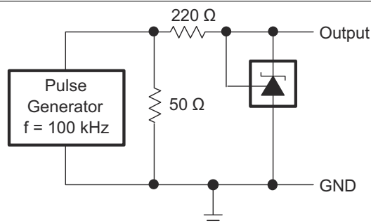
Figure 7-15. Test Circuit for Pulse Response
