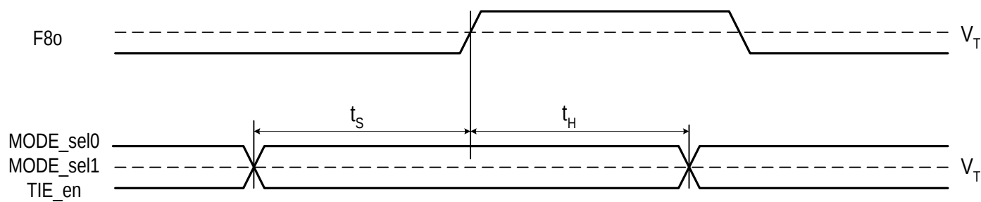
Figure - 15 Input Control Setup and Hold Timing
