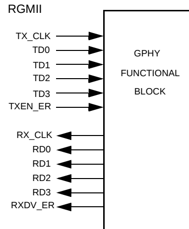
Figure 5. RGMII Signals
