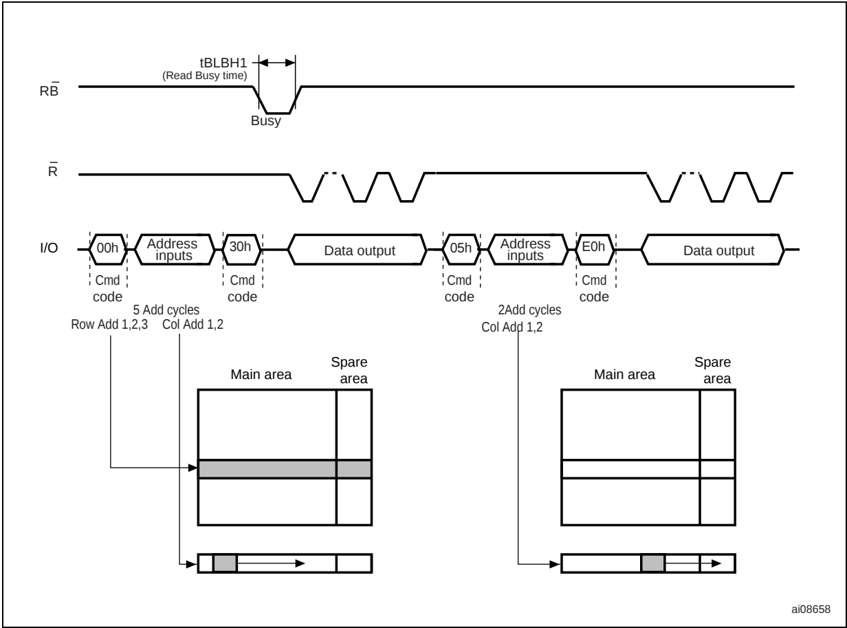
Figure 7. Random data output during sequential data output
